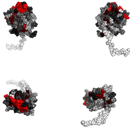
Fig. 2. Residues in 2diyA, colored by their relative importance. Clockwise: front, back, top and bottom views.
