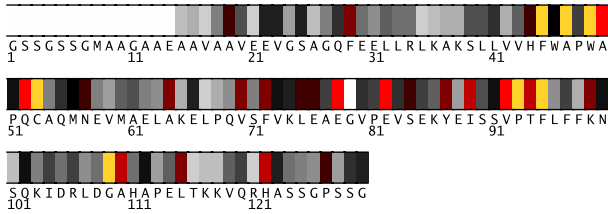
Fig. 1. Residues 1-130 in 2diyA colored by their relative importance. (See Appendix, Fig.5, for the coloring scheme.)
