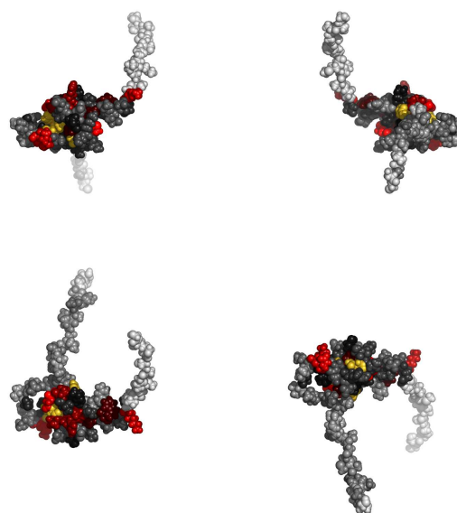
Fig. 2. Residues in 2dklA, colored by their relative importance. Clockwise: front, back, top and bottom views.
