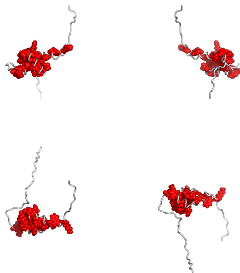
Fig. 3. Residues in 2dklA, colored according to the cluster they belong to: red, followed by blue and yellow are the largest clusters (see Appendix for the coloring scheme). Clockwise: front, back, top and bottom views. The corresponding Pymol script is attached.
