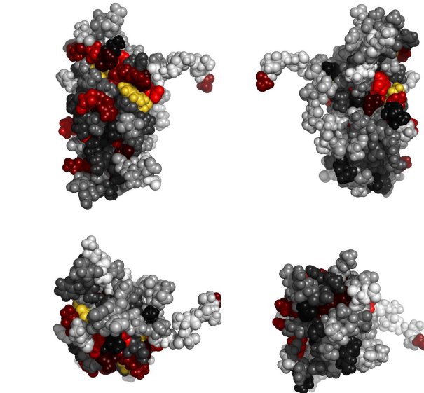
Fig. 1. Residues 1-142 in 2dmgA colored by their relative importance. (See Appendix, Fig.5, for the coloring scheme.)
