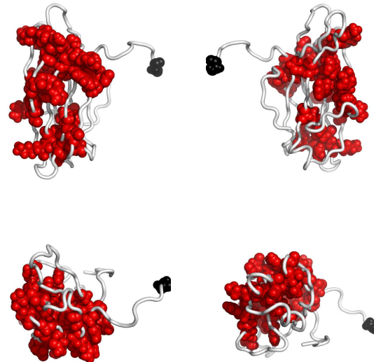
Fig. 2. Residues in 2dmgA, colored by their relative importance. Clockwise: front, back, top and bottom views.
