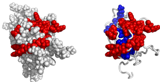
Fig. 4. A possible active surface on the chain 2dmgA. The larger cluster it belongs to is shown in blue.
