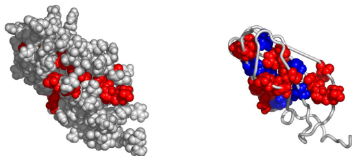
Fig. 4. A possible active surface on the chain 2ds4A. The larger cluster it belongs to is shown in blue.
