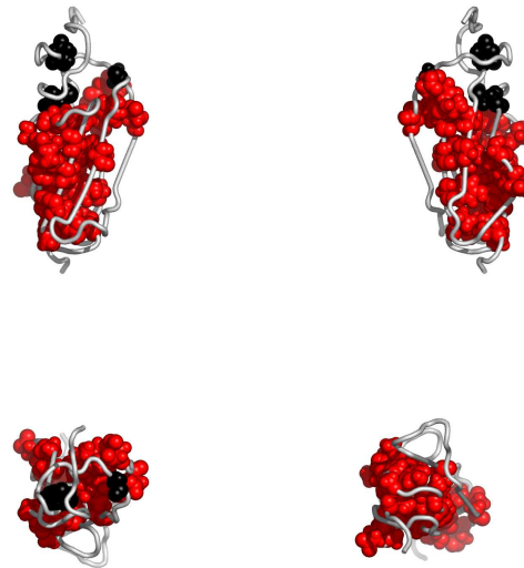
Fig. 2. Residues in 2ds4A, colored by their relative importance. Clockwise: front, back, top and bottom views.
