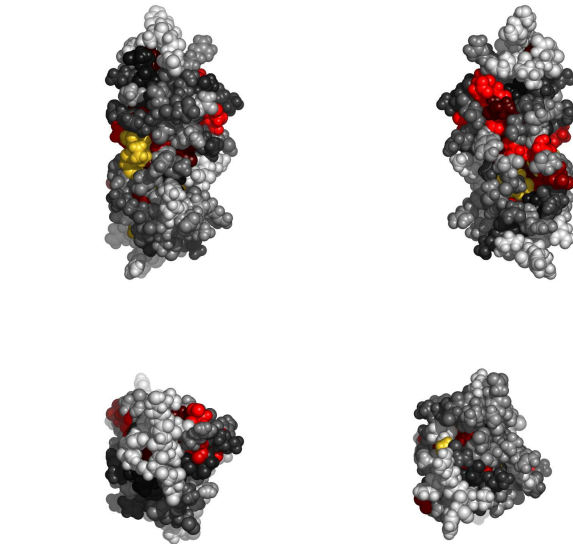
Fig. 1. Residues 1-113 in 2ds4A colored by their relative importance. (See Appendix, Fig.5, for the coloring scheme.)
