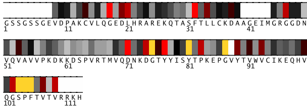
Fig. 1. Residues 1-113 in 2ds4A colored by their relative importance. (See Appendix, Fig.5, for the coloring scheme.)
