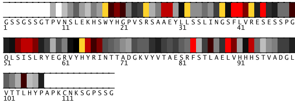
Fig. 1. Residues 1-119 in 2ecdA colored by their relative importance. (See Appendix, Fig.5, for the coloring scheme.)
