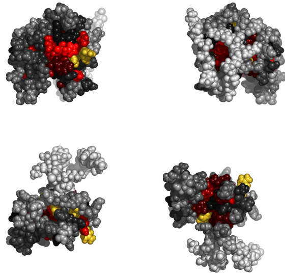
Fig. 2. Residues in 2ecdA, colored by their relative importance. Clockwise: front, back, top and bottom views.
