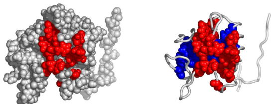
Fig. 4. A possible active surface on the chain 2ecdA. The larger cluster it belongs to is shown in blue.
