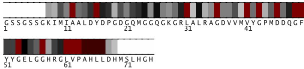
Fig. 1. Residues 1-75 in 2egeA colored by their relative importance. (See Appendix, Fig.5, for the coloring scheme.)
