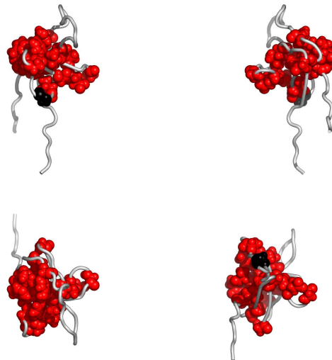
Fig. 3. Residues in 2egeA, colored according to the cluster they belong to: red, followed by blue and yellow are the largest clusters (see Appendix for the coloring scheme). Clockwise: front, back, top and bottom views. The corresponding Pymol script is attached.
