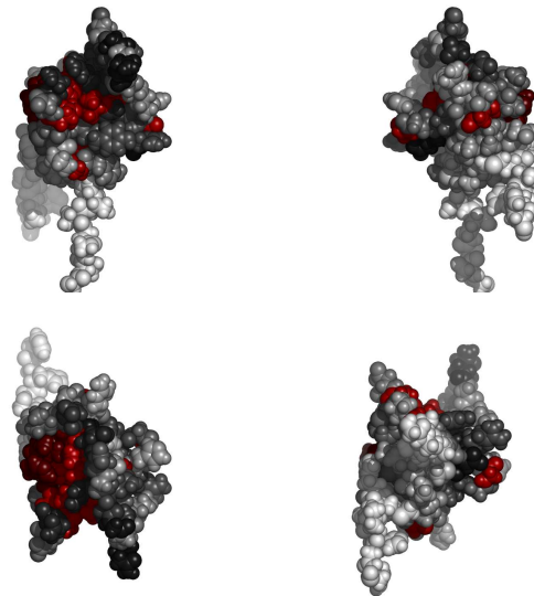
Fig. 2. Residues in 2egeA, colored by their relative importance. Clockwise: front, back, top and bottom views.
