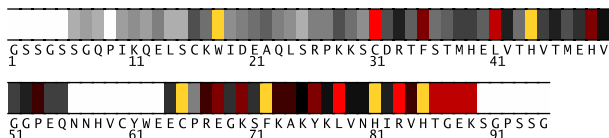
Fig. 1. Residues 1-95 in 2ej4A colored by their relative importance. (See Appendix, Fig.7, for the coloring scheme.)
