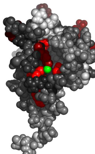
Fig. 5. Residues in 2ej4A, at the interface with zinc ion, colored by their relative importance. The ligand (zinc ion) is colored green. Atoms further than 30Å away from the geometric center of the ligand, as well as on the line of sight to the ligand were removed. (See Appendix for the coloring scheme for the protein chain 2ej4A.)
