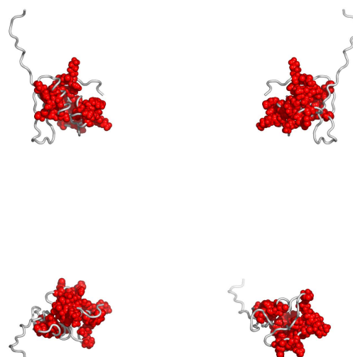
Fig. 2. Residues in 2ej4A, colored by their relative importance. Clockwise: front, back, top and bottom views.
