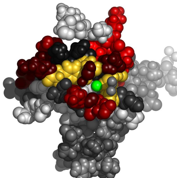
Fig. 4. Residues in 2ej4A, at the interface with zinc ion, colored by their relative importance. The ligand (zinc ion) is colored green. Atoms further than 30Å away from the geometric center of the ligand, as well as on the line of sight to the ligand were removed. (See Appendix for the coloring scheme for the protein chain 2ej4A.)
