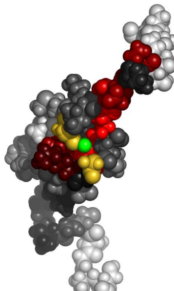
Fig. 4. Residues in 2emfA, at the interface with zinc ion, colored by their relative importance. The ligand (zinc ion) is colored green. Atoms further than 30Å away from the geometric center of the ligand, as well as on the line of sight to the ligand were removed. (See Appendix for the coloring scheme for the protein chain 2emfA.)
