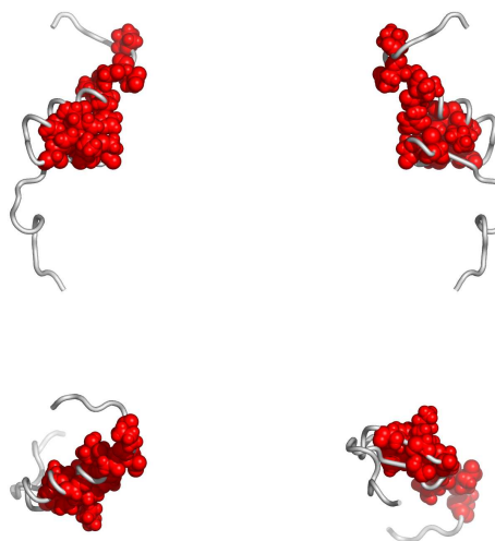
Fig. 2. Residues in 2emfA, colored by their relative importance. Clockwise: front, back, top and bottom views.
