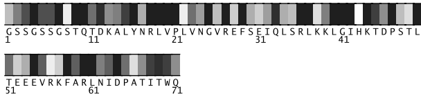
Fig. 1. Residues 1-71 in 2eo2A colored by their relative importance. (See Appendix, Fig.4, for the coloring scheme.)
