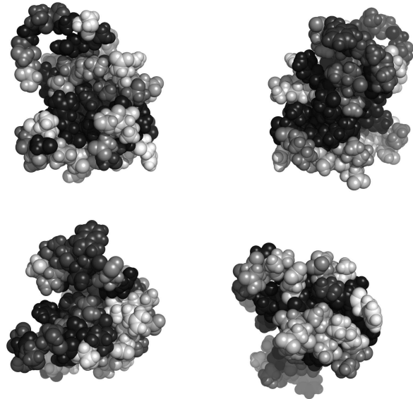
Fig. 2. Residues in 2eo2A, colored by their relative importance. Clockwise: front, back, top and bottom views.
