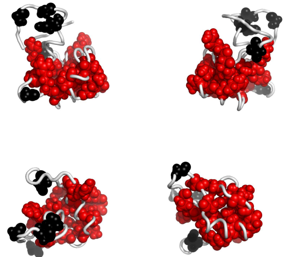
Fig. 2. Residues in 2eo2A, colored by their relative importance. Clockwise: front, back, top and bottom views.
