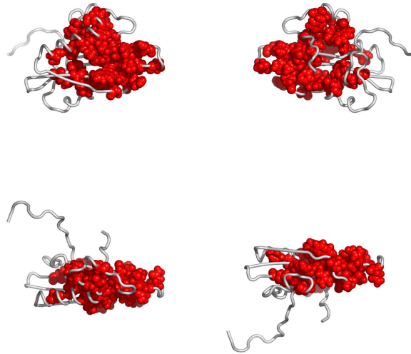
Fig. 3. Residues in 2eocA, colored according to the cluster they belong to: red, followed by blue and yellow are the largest clusters (see Appendix for the coloring scheme). Clockwise: front, back, top and bottom views. The corresponding Pymol script is attached.
