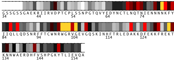
Fig. 1. Residues 34-157 in 2eocA colored by their relative importance. (See Appendix, Fig.5, for the coloring scheme.)
