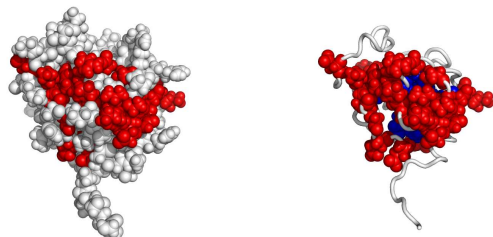
Fig. 4. A possible active surface on the chain 2eqoA. The larger cluster it belongs to is shown in blue.
