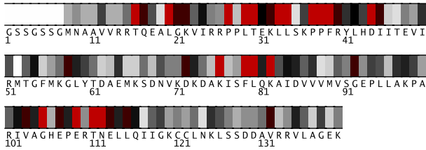
Fig. 1. Residues 1-140 in 2eqoA colored by their relative importance. (See Appendix, Fig.5, for the coloring scheme.)
