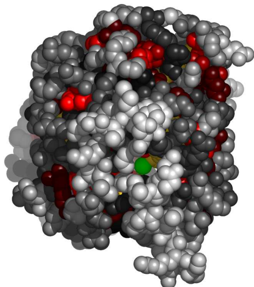
Fig. 6. Residues in 2ffuA, at the interface with manganese (ii) ion, colored by their relative importance. The ligand (manganese (ii) ion) is colored green. Atoms further than 30 Å away from the geometric center of the ligand, as well as on the line of sight to the ligand were removed. (See Appendix for the coloring scheme for the protein chain 2ffuA.)
