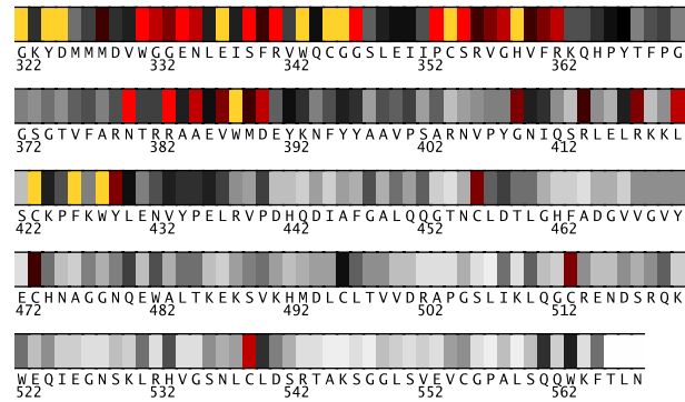
Fig. 2. Residues 322-568 in 2ffuA colored by their relative importance. (See Appendix, Fig.9, for the coloring scheme.)
