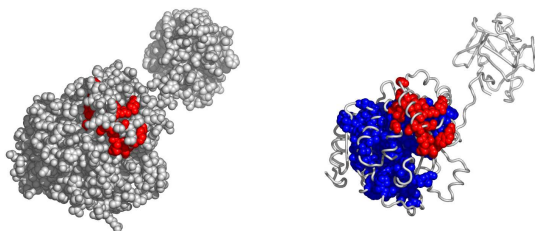
Fig. 8. A possible active surface on the chain 2ffuA. The larger cluster it belongs to is shown in blue.
