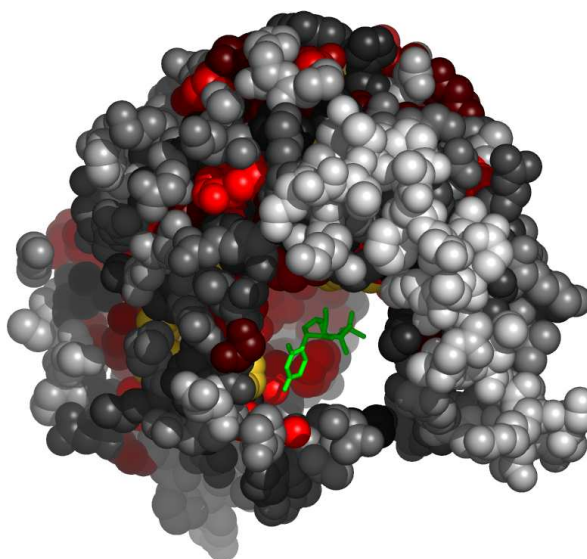
Fig. 5. Residues in 2ffuA, at the interface with UDP, colored by their relative importance. The ligand (UDP) is colored green. Atoms further than 30 Å away from the geometric center of the ligand, as well as on the line of sight to the ligand were removed. (See Appendix for the coloring scheme for the protein chain 2ffuA.)
