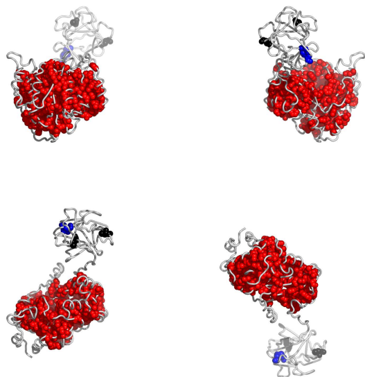
Fig. 4. Residues in 2ffuA, colored according to the cluster they belong to: red, followed by blue and yellow are the largest clusters (see Appendix for the coloring scheme). Clockwise: front, back, top and bottom views. The corresponding Pymol script is attached.
