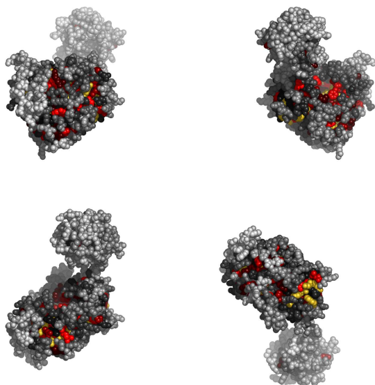
Fig. 3. Residues in 2ffuA, colored by their relative importance. Clockwise: front, back, top and bottom views.
