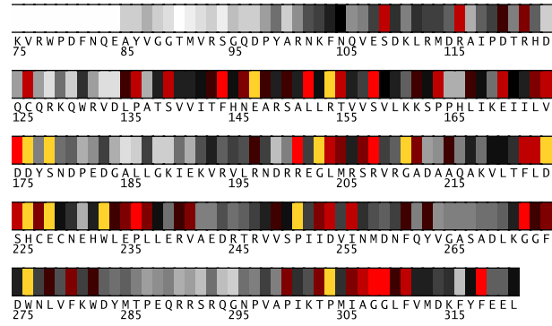
Fig. 1. Residues 75-321 in 2ffuA colored by their relative importance. (See Appendix, Fig.9, for the coloring scheme.)
