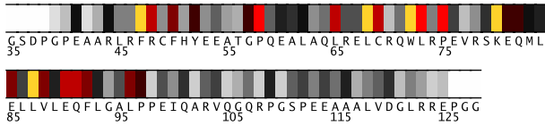
Fig. 1. Residues 35-128 in 2fi2A colored by their relative importance. (See Appendix, Fig.5, for the coloring scheme.)
