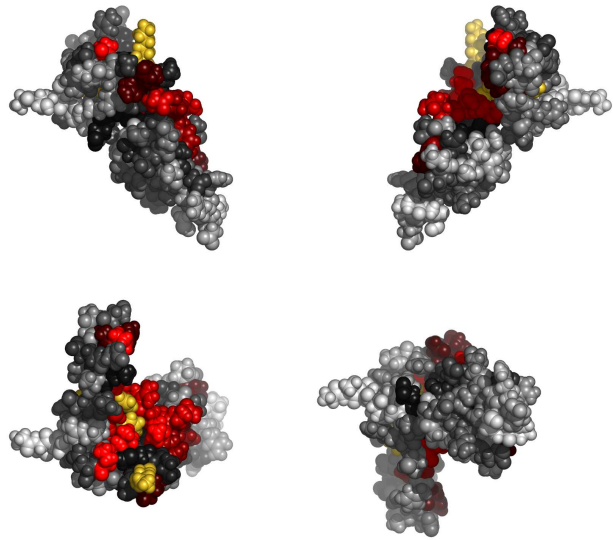
Fig. 2. Residues in 2fi2A, colored by their relative importance. Clockwise: front, back, top and bottom views.
