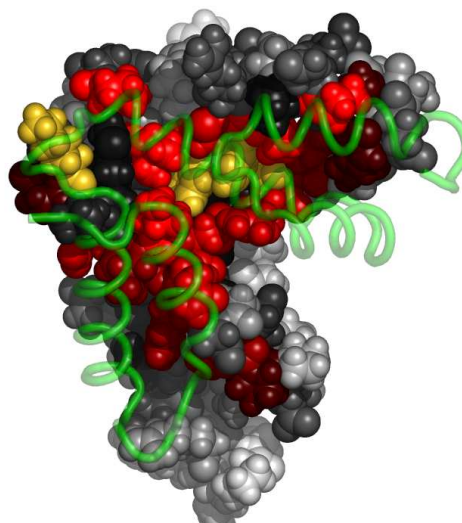
Fig. 4. Residues in 2fi2A, at the interface with 2fi2B, colored by their relative importance. 2fi2B is shown in backbone representation (See Appendix for the coloring scheme for the protein chain 2fi2A.)
