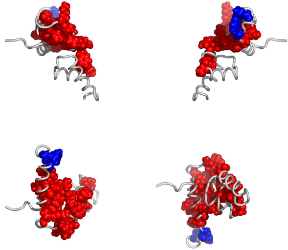
Fig. 3. Residues in 2fi2A, colored according to the cluster they belong to: red, followed by blue and yellow are the largest clusters (see Appendix for the coloring scheme). Clockwise: front, back, top and bottom views. The corresponding Pymol script is attached.
