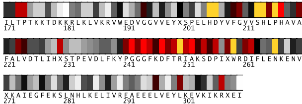
Fig. 2. Residues 171-310 in 2g5cB colored by their relative importance. (See Appendix, Fig.8, for the coloring scheme.)
