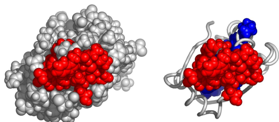
Fig. 4. A possible active surface on the chain 2gzyA. The larger cluster it belongs to is shown in blue.
