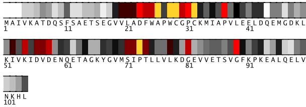
Fig. 1. Residues 1-104 in 2gzyA colored by their relative importance. (See Appendix, Fig.5, for the coloring scheme.)
