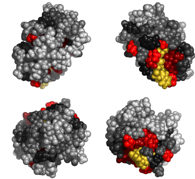
Fig. 2. Residues in 2gzyA, colored by their relative importance. Clockwise: front, back, top and bottom views.
