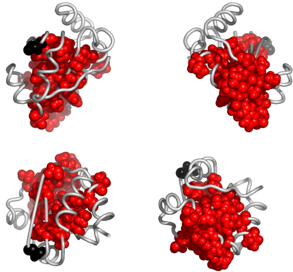
Fig. 3. Residues in 2gzyA, colored according to the cluster they belong to: red, followed by blue and yellow are the largest clusters (see Appendix for the coloring scheme). Clockwise: front, back, top and bottom views. The corresponding Pymol script is attached.
