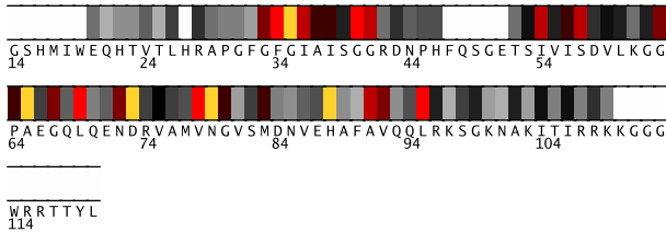
Fig. 1. Residues 14-120 in 2h2bA colored by their relative importance. (See Appendix, Fig.6, for the coloring scheme.)
