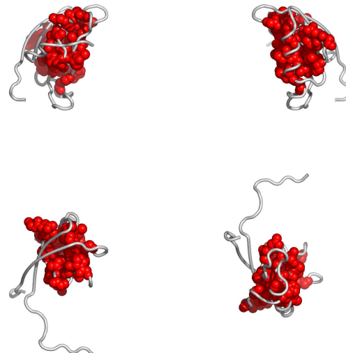
Fig. 3. Residues in 2h2bA, colored according to the cluster they belong to: red, followed by blue and yellow are the largest clusters (see Appendix for the coloring scheme). Clockwise: front, back, top and bottom views. The corresponding Pymol script is attached.
