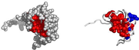
Fig. 5. A possible active surface on the chain 2h2bA. The larger cluster it belongs to is shown in blue.
