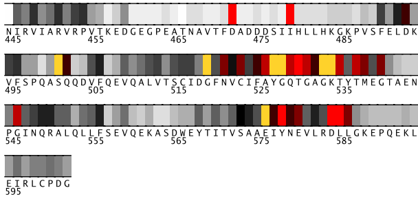
Fig. 1. Residues 445-602 in 2h58A colored by their relative importance. (See Appendix, Fig.12, for the coloring scheme.)
