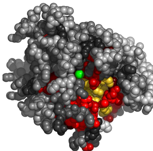
Fig. 8. Residues in 2h58A, at the interface with unknown atom or ion, colored by their relative importance. The ligand (unknown atom or ion) is colored green. Atoms further than 30\text{\AA} away from the geometric center of the ligand, as well as on the line of sight to the ligand were removed. (See Appendix for the coloring scheme for the protein chain 2h58A.)
