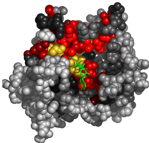
Fig. 10. Residues in 2h58A, at the interface with ADP, colored by their relative importance. The ligand (ADP) is colored green. Atoms further than 30\text{\AA} away from the geometric center of the ligand, as well as on the line of sight to the ligand were removed. (See Appendix for the coloring scheme for the protein chain 2h58A.)
