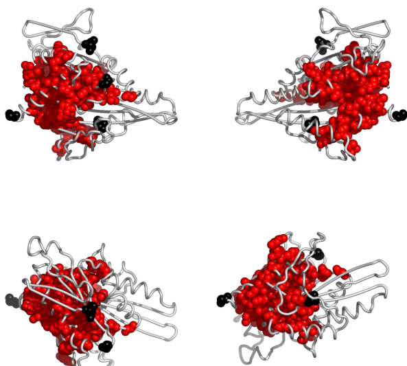
Fig. 4. Residues in 2h58A, colored according to the cluster they belong to: red, followed by blue and yellow are the largest clusters (see Appendix for the coloring scheme). Clockwise: front, back, top and bottom views. The corresponding Pymol script is attached.
