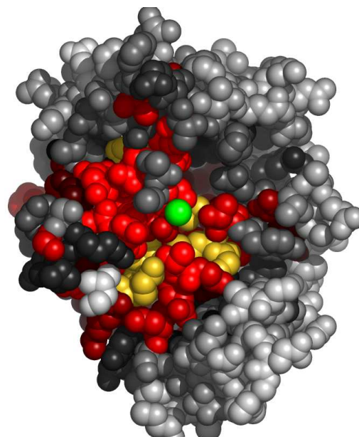
Fig. 6. Residues in 2h58A, at the interface with unknown atom or ion, colored by their relative importance. The ligand (unknown atom or ion) is colored green. Atoms further than 30 Å away from the geometric center of the ligand, as well as on the line of sight to the ligand were removed. (See Appendix for the coloring scheme for the protein chain 2h58A.)
