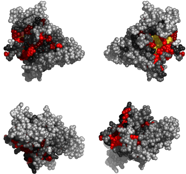
Fig. 3. Residues in 2h58A, colored by their relative importance. Clockwise: front, back, top and bottom views.
