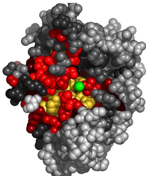
Fig. 7. Residues in 2h58A, at the interface with magnesium ion, colored by their relative importance. The ligand (magnesium ion) is colored green. Atoms further than 30\text{\AA} away from the geometric center of the ligand, as well as on the line of sight to the ligand were removed. (See Appendix for the coloring scheme for the protein chain 2h58A.)
