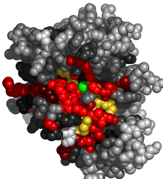
Fig. 5. Residues in 2h58A, at the interface with unknown atom or ion, colored by their relative importance. The ligand (unknown atom or ion) is colored green. Atoms further than 30 Å away from the geometric center of the ligand, as well as on the line of sight to the ligand were removed. (See Appendix for the coloring scheme for the protein chain 2h58A.)
