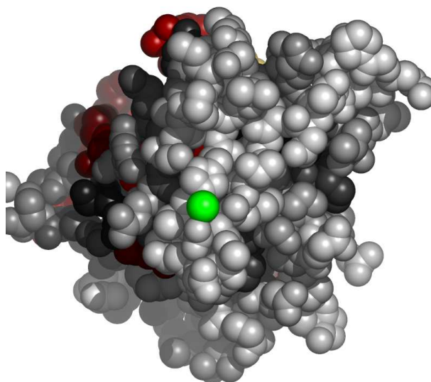
Fig. 11. Residues in 2h58A, at the interface with unknown atom or ion, colored by their relative importance. The ligand (unknown atom or ion) is colored green. Atoms further than 30\text{\AA} away from the geometric center of the ligand, as well as on the line of sight to the ligand were removed. (See Appendix for the coloring scheme for the protein chain 2h58A.)
