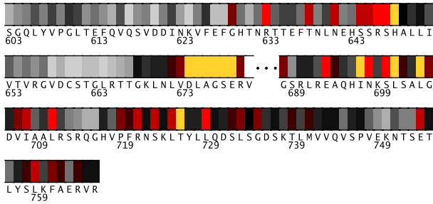
Fig. 2. Residues 603-766 in 2h58A colored by their relative importance. (See Appendix, Fig.12, for the coloring scheme.)
