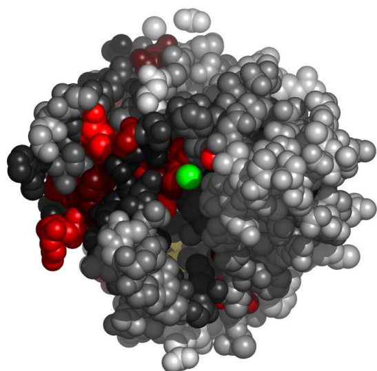
Fig. 9. Residues in 2h58A, at the interface with unknown atom or ion, colored by their relative importance. The ligand (unknown atom or ion) is colored green. Atoms further than 30Å away from the geometric center of the ligand, as well as on the line of sight to the ligand were removed. (See Appendix for the coloring scheme for the protein chain 2h58A.)
