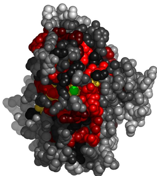
Fig. 7. Residues in 2hd1A, at the interface with magnesium ion, colored by their relative importance. The ligand (magnesium ion) is colored green. Atoms further than 30Å away from the geometric center of the ligand, as well as on the line of sight to the ligand were removed. (See Appendix for the coloring scheme for the protein chain 2hd1A.)
