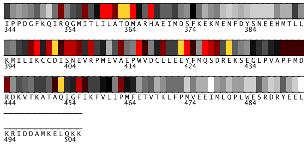
Fig. 2. Residues 344-506 in 2hd1A colored by their relative importance. (See Appendix, Fig.10, for the coloring scheme.)
