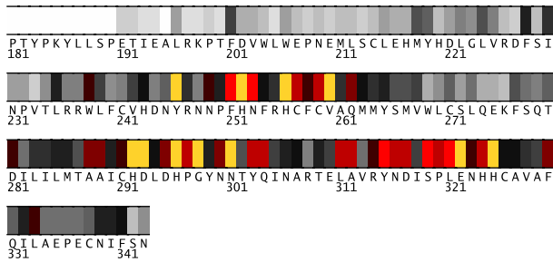
Fig. 1. Residues 181-343 in 2hd1A colored by their relative importance. (See Appendix, Fig.10, for the coloring scheme.)
