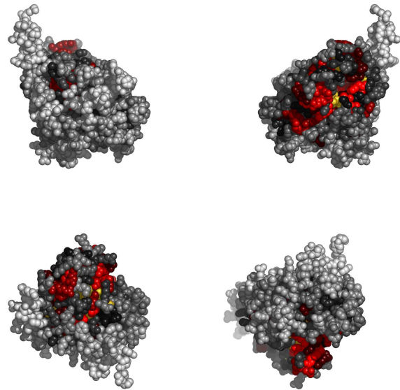
Fig. 3. Residues in 2hd1A, colored by their relative importance. Clockwise: front, back, top and bottom views.
