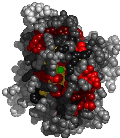
Fig. 5. Residues in 2hd1A, at the interface with zinc ion, colored by their relative importance. The ligand (zinc ion) is colored green. Atoms further than 30Å away from the geometric center of the ligand, as well as on the line of sight to the ligand were removed. (See Appendix for the coloring scheme for the protein chain 2hd1A.)
