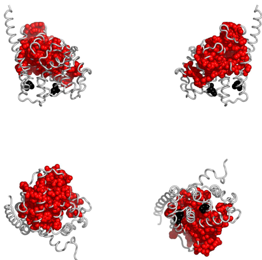
Fig. 4. Residues in 2hd1A, colored according to the cluster they belong to: red, followed by blue and yellow are the largest clusters (see Appendix for the coloring scheme). Clockwise: front, back, top and bottom views. The corresponding Pymol script is attached.
