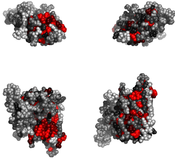
Fig. 3. Residues in 2hz6A, colored by their relative importance. Clockwise: front, back, top and bottom views.
