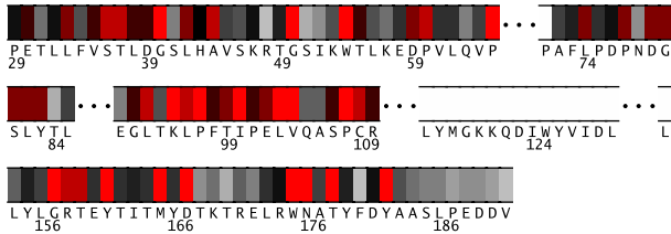
Fig. 1. Residues 29-191 in 2hz6A colored by their relative importance. (See Appendix, Fig.7, for the coloring scheme.)
