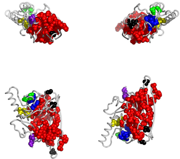
Fig. 4. Residues in 2hz6A, colored according to the cluster they belong to: red, followed by blue and yellow are the largest clusters (see Appendix for the coloring scheme). Clockwise: front, back, top and bottom views. The corresponding Pymol script is attached.
