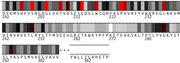
Fig. 2. Residues 192-368 in 2hz6A colored by their relative importance. (See Appendix, Fig.7, for the coloring scheme.)
