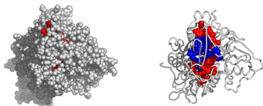
Fig. 9. A possible active surface on the chain 2io7A. The larger cluster it belongs to is shown in blue.
