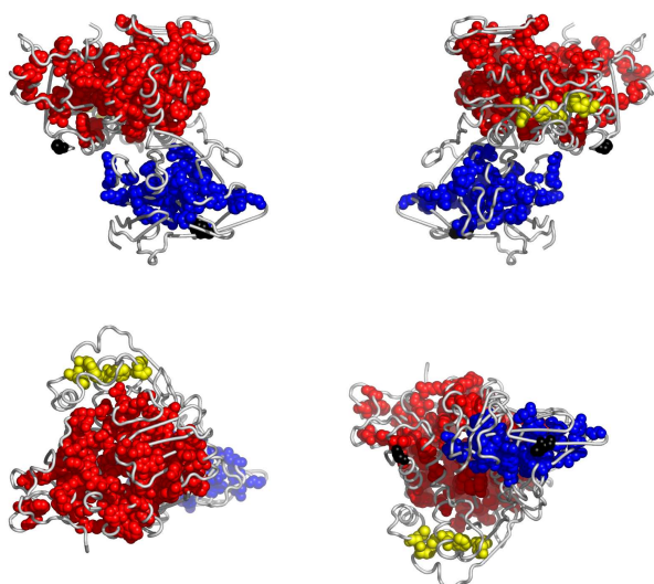
Fig. 4. Residues in 2io7A, colored according to the cluster they belong to: red, followed by blue and yellow are the largest clusters (see Appendix for the coloring scheme). Clockwise: front, back, top and bottom views. The corresponding Pymol script is attached.
