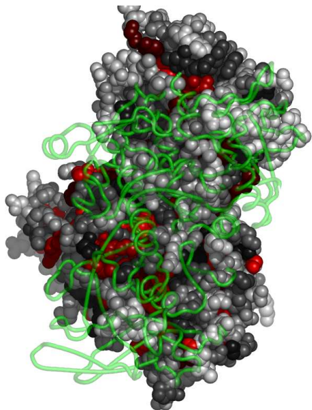
Fig. 7. Residues in 2io7A, at the interface with 2io7B, colored by their relative importance. 2io7B is shown in backbone representation (See Appendix for the coloring scheme for the protein chain 2io7A.)
