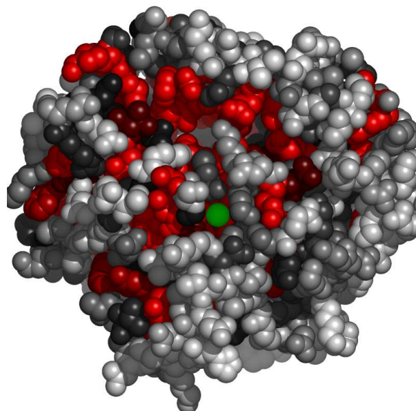
Fig. 6. Residues in 2io7A, at the interface with magnesium ion, colored by their relative importance. The ligand (magnesium ion) is colored green. Atoms further than 30Å away from the geometric center of the ligand, as well as on the line of sight to the ligand were removed. (See Appendix for the coloring scheme for the protein chain 2io7A.)
