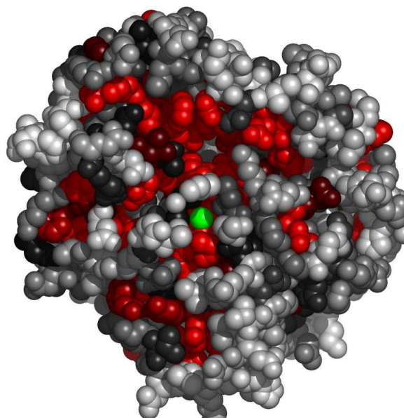
Fig. 5. Residues in 2io7A, at the interface with magnesium ion, colored by their relative importance. The ligand (magnesium ion) is colored green. Atoms further than 30 Å away from the geometric center of the ligand, as well as on the line of sight to the ligand were removed. (See Appendix for the coloring scheme for the protein chain 2io7A.)
