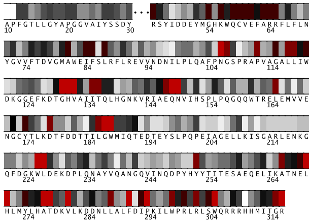
Fig. 1. Residues 10-316 in 2io7A colored by their relative importance. (See Appendix, Fig.10, for the coloring scheme.)
