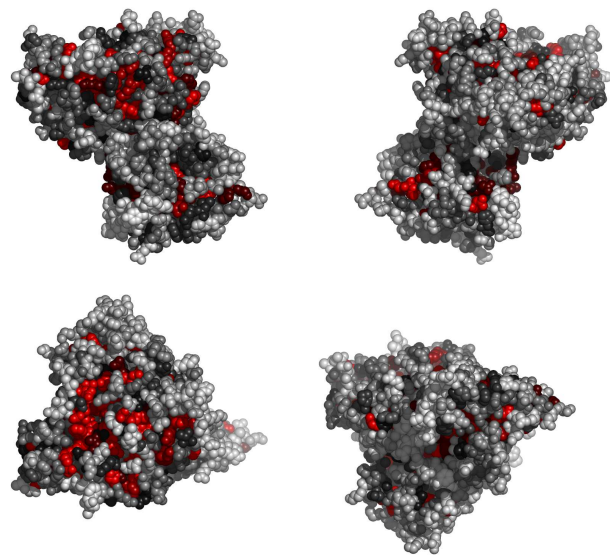
Fig. 3. Residues in 2io7A, colored by their relative importance. Clockwise: front, back, top and bottom views.
