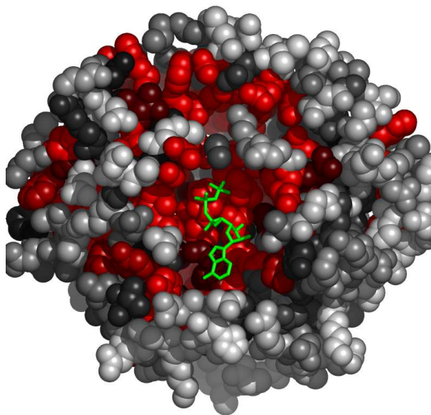
Fig. 8. Residues in 2io7A, at the interface with ANP, colored by their relative importance. The ligand (ANP) is colored green. Atoms further than 30 Å away from the geometric center of the ligand, as well as on the line of sight to the ligand were removed. (See Appendix for the coloring scheme for the protein chain 2io7A.)
