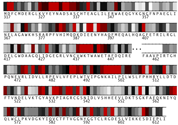
Fig. 2. Residues 317-615 in 2io7A colored by their relative importance. (See Appendix, Fig.10, for the coloring scheme.)
