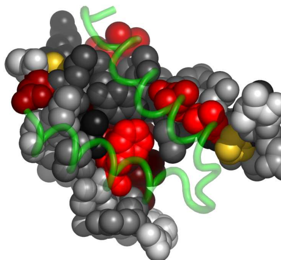
Fig. 4. Residues in 2izxB, at the interface with 2izxA, colored by their relative importance. 2izxA is shown in backbone representation (See Appendix for the coloring scheme for the protein chain 2izxB.)
