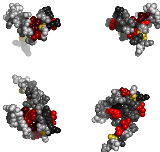
Fig. 2. Residues in 2ixzB, colored by their relative importance. Clockwise: front, back, top and bottom views.
