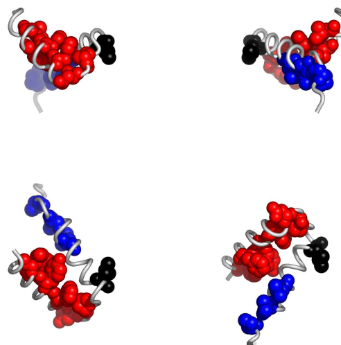
Fig. 3. Residues in 2ixzB, colored according to the cluster they belong to: red, followed by blue and yellow are the largest clusters (see Appendix for the coloring scheme). Clockwise: front, back, top and bottom views. The corresponding Pymol script is attached.
