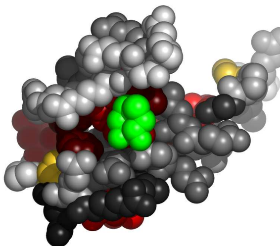
Fig. 5. Residues in 2izxB, at the interface with dithiane diol, colored by their relative importance. The ligand (dithiane diol) is colored green. Atoms further than 30Å away from the geometric center of the ligand, as well as on the line of sight to the ligand were removed. (See Appendix for the coloring scheme for the protein chain 2izxB.)
