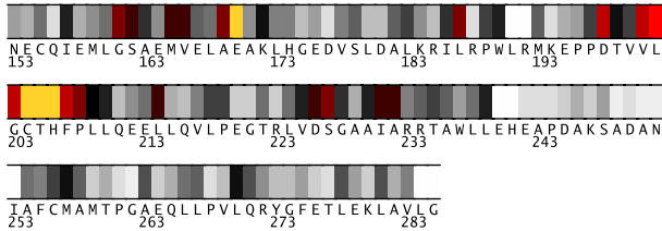
Fig. 2. Residues 153-285 in 2jfnA colored by their relative importance. (See Appendix, Fig.7, for the coloring scheme.)
