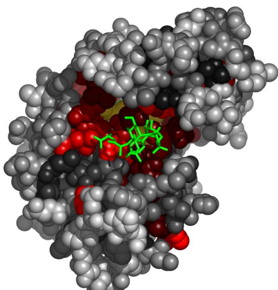
Fig. 5. Residues in 2jfnA, at the interface with UMA, colored by their relative importance. The ligand (UMA) is colored green. Atoms further than 30Å away from the geometric center of the ligand, as well as on the line of sight to the ligand were removed. (See Appendix for the coloring scheme for the protein chain 2jfnA.)
