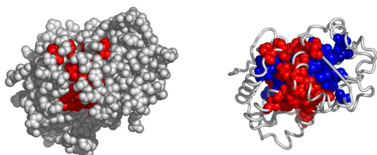
Fig. 6. A possible active surface on the chain 2jfnA. The larger cluster it belongs to is shown in blue.
