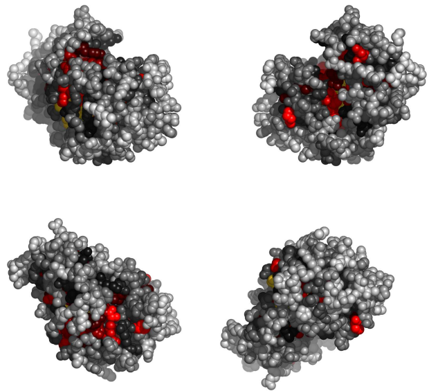
Fig. 3. Residues in 2jfnA, colored by their relative importance. Clockwise: front, back, top and bottom views.
