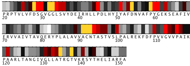
Fig. 1. Residues 20-152 in 2jfnA colored by their relative importance. (See Appendix, Fig.7, for the coloring scheme.)
