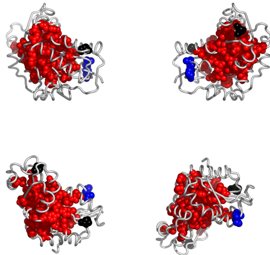
Fig. 4. Residues in 2jfnA, colored according to the cluster they belong to: red, followed by blue and yellow are the largest clusters (see Appendix for the coloring scheme). Clockwise: front, back, top and bottom views. The corresponding Pymol script is attached.
