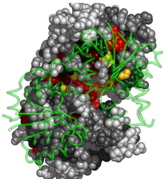
Fig. 7. Residues in 2jjmA, at the interface with 2jjmB, colored by their relative importance. 2jjmB is shown in backbone representation (See Appendix for the coloring scheme for the protein chain 2jjmA.)
