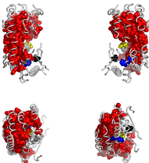
Fig. 4. Residues in 2jjmA, colored according to the cluster they belong to: red, followed by blue and yellow are the largest clusters (see Appendix for the coloring scheme). Clockwise: front, back, top and bottom views. The corresponding Pymol script is attached.
