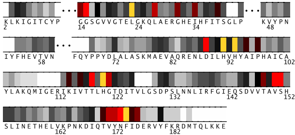
Fig. 1. Residues 2-191 in 2jjmA colored by their relative importance. (See Appendix, Fig.9, for the coloring scheme.)
