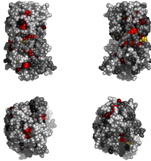
Fig. 3. Residues in 2jjmA, colored by their relative importance. Clockwise: front, back, top and bottom views.
