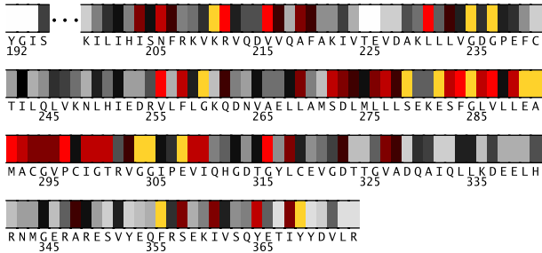
Fig. 2. Residues 192-374 in 2jjmA colored by their relative importance. (See Appendix, Fig.9, for the coloring scheme.)
