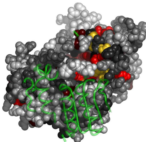
Fig. 4. Residues in 2jjmA, colored according to the cluster they belong to: red, followed by blue and yellow are the largest clusters (see Appendix for the coloring scheme). Clockwise: front, back, top and bottom views. The corresponding Pymol script is attached.
