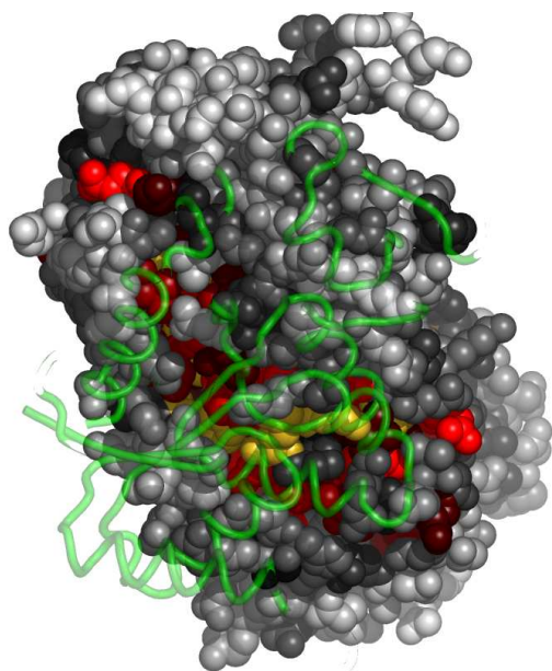
Fig. 6. Residues in 2jjmA, at the interface with 2jjmC, colored by their relative importance. 2jjmC is shown in backbone representation (See Appendix for the coloring scheme for the protein chain 2jjmA.)
