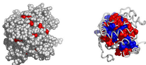
Fig. 8. A possible active surface on the chain 2jjmA. The larger cluster it belongs to is shown in blue.
