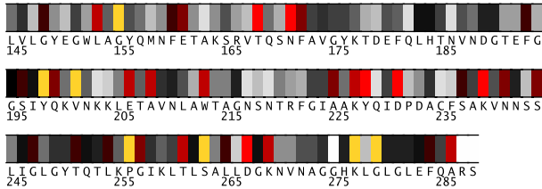
Fig. 2. Residues 145-288 in 2jk4A colored by their relative importance. (See Appendix, Fig.9, for the coloring scheme.)
