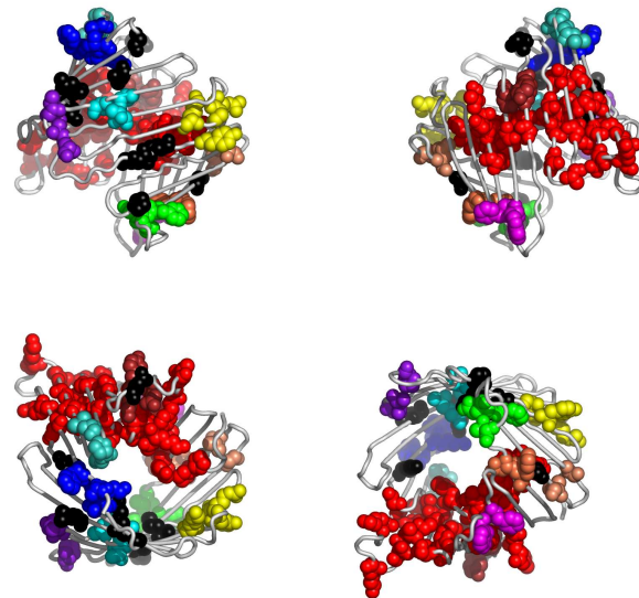
Fig. 4. Residues in 2jk4A, colored according to the cluster they belong to: red, followed by blue and yellow are the largest clusters (see Appendix for the coloring scheme). Clockwise: front, back, top and bottom views. The corresponding Pymol script is attached.
