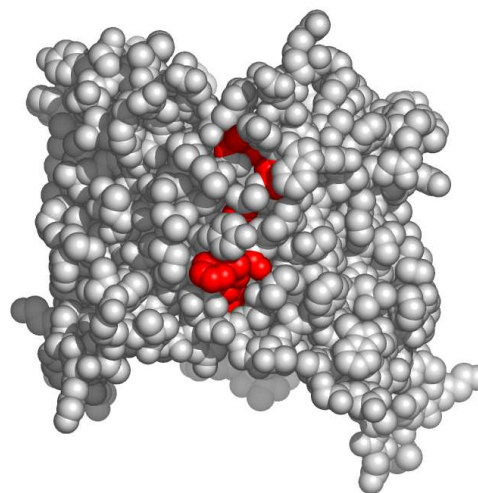
Fig. 6. Another possible active surface on the chain 2jk4A.
