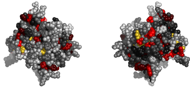
Fig. 1. Residues 1-144 in 2jk4A colored by their relative importance. (See Appendix, Fig.9, for the coloring scheme.)
