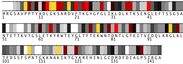
Fig. 1. Residues 1-144 in 2jk4A colored by their relative importance. (See Appendix, Fig.9, for the coloring scheme.)
