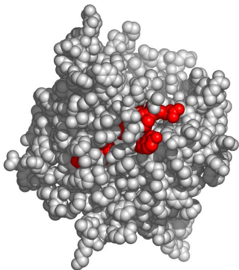
Fig. 5. A possible active surface on the chain 2jk4A.
