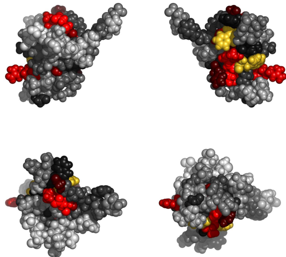
Fig. 2. Residues in 2k1bA, colored by their relative importance. Clockwise: front, back, top and bottom views.
