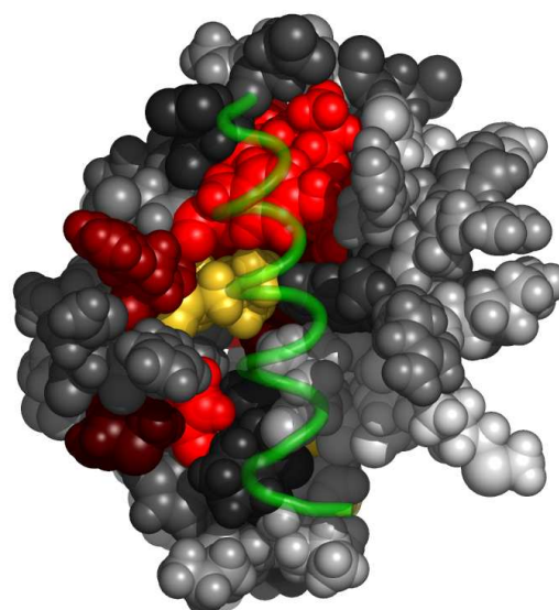
Fig. 4. Residues in 2kbrA, at the interface with 2kbrB, colored by their relative importance. 2kbrB is shown in backbone representation (See Appendix for the coloring scheme for the protein chain 2kbrA.)
