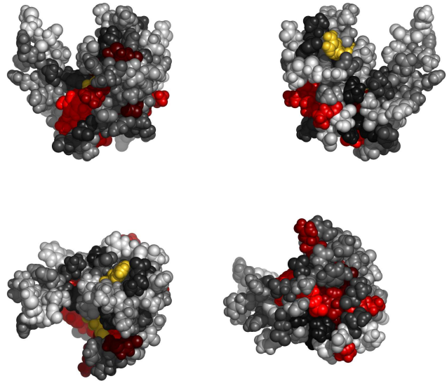
Fig. 2. Residues in 2kbrA, colored by their relative importance. Clockwise: front, back, top and bottom views.
