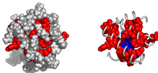
Fig. 5. A possible active surface on the chain 2kbrA. The larger cluster it belongs to is shown in blue.
