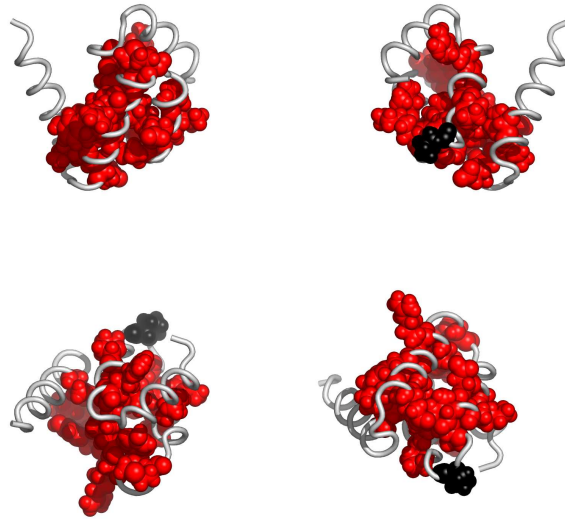
Fig. 3. Residues in 2kbrA, colored according to the cluster they belong to: red, followed by blue and yellow are the largest clusters (see Appendix for the coloring scheme). Clockwise: front, back, top and bottom views. The corresponding Pymol script is attached.
