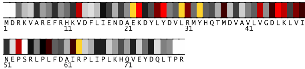
Fig. 1. Residues 1-80 in 2kbrA colored by their relative importance. (See Appendix, Fig.6, for the coloring scheme.)
