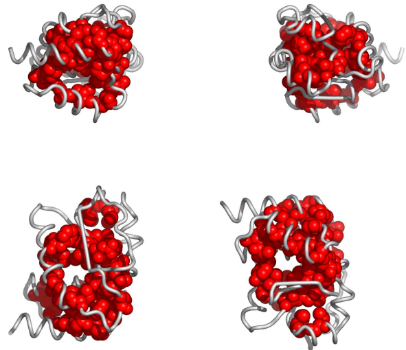
Fig. 3. Residues in 2nt2A, colored according to the cluster they belong to: red, followed by blue and yellow are the largest clusters (see Appendix for the coloring scheme). Clockwise: front, back, top and bottom views. The corresponding Pymol script is attached.
