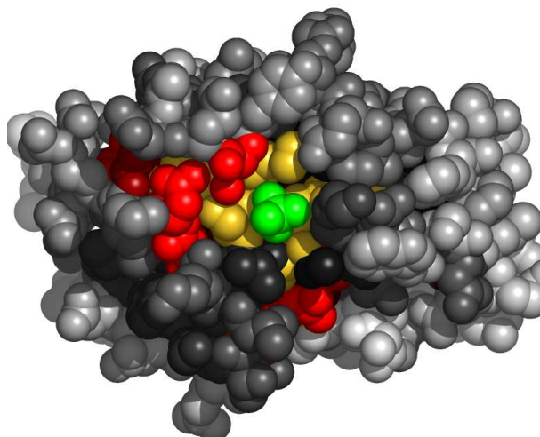
Fig. 4. Residues in 2nt2A, at the interface with sulfate ion, colored by their relative importance. The ligand (sulfate ion) is colored green. Atoms further than 30Å away from the geometric center of the ligand, as well as on the line of sight to the ligand were removed. (See Appendix for the coloring scheme for the protein chain 2nt2A.)
