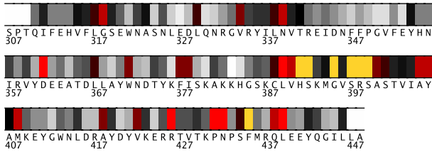
Fig. 1. Residues 307-448 in 2nt2A colored by their relative importance. (See Appendix, Fig.6, for the coloring scheme.)
