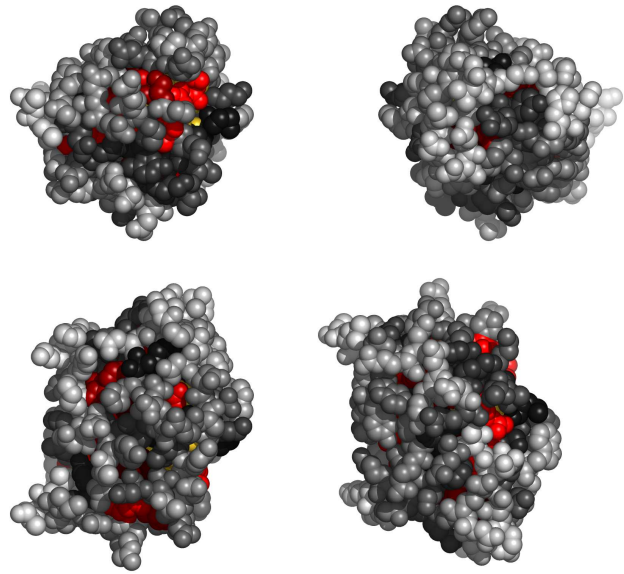
Fig. 2. Residues in 2nt2A, colored by their relative importance. Clockwise: front, back, top and bottom views.
