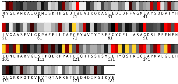
Fig. 1. Residues 1-182 in 2o09A colored by their relative importance. (See Appendix, Fig.7, for the coloring scheme.)
