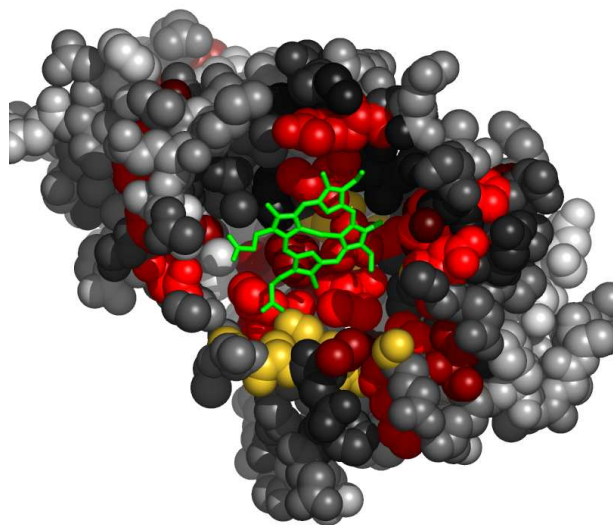
Fig. 4. Residues in 2o09A, at the interface with HEM, colored by their relative importance. The ligand (HEM) is colored green. Atoms further than 30Å away from the geometric center of the ligand, as well as on the line of sight to the ligand were removed. (See Appendix for the coloring scheme for the protein chain 2o09A.)
