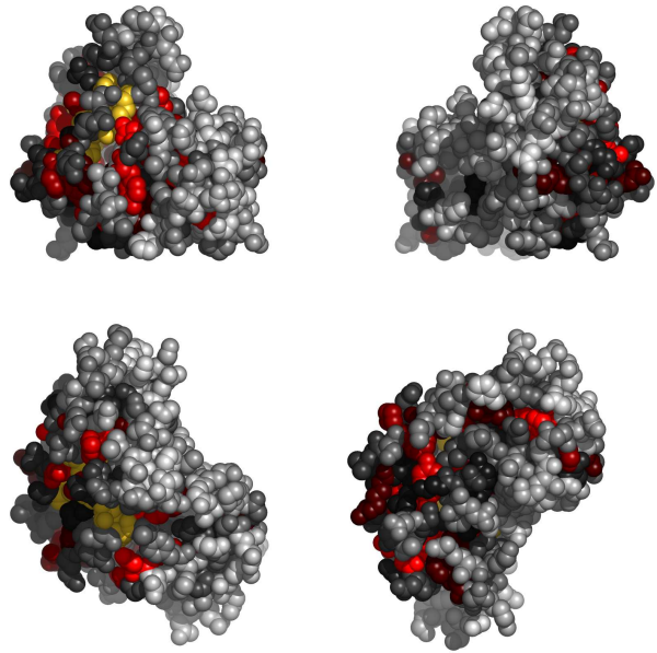
Fig. 2. Residues in 2o09A, colored by their relative importance. Clockwise: front, back, top and bottom views.
