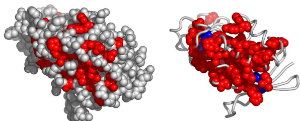
Fig. 6. A possible active surface on the chain 2o09A. The larger cluster it belongs to is shown in blue.
