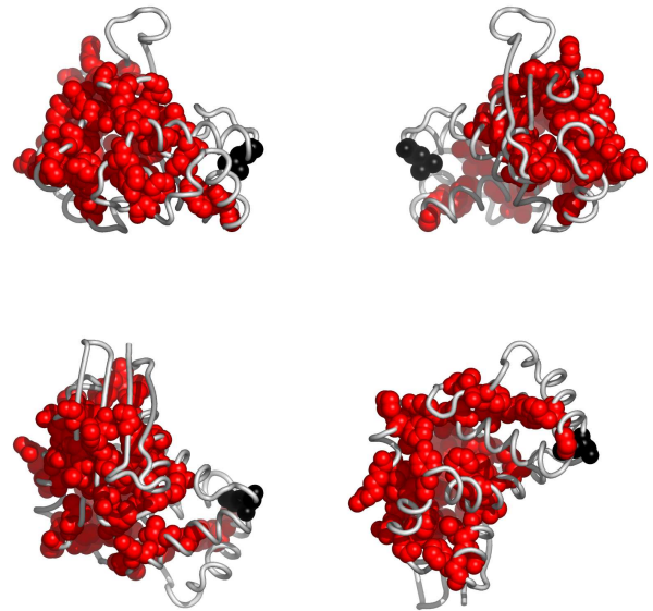
Fig. 3. Residues in 2o09A, colored according to the cluster they belong to: red, followed by blue and yellow are the largest clusters (see Appendix for the coloring scheme). Clockwise: front, back, top and bottom views. The corresponding Pymol script is attached.
