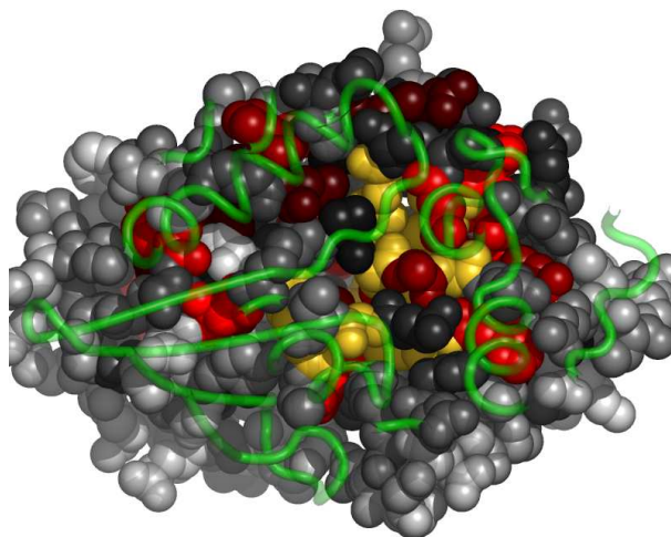
Fig. 4. Residues in 2o09A, at the interface with HEM, colored by their relative importance. The ligand (HEM) is colored green. Atoms further than 30Å away from the geometric center of the ligand, as well as on the line of sight to the ligand were removed. (See Appendix for the coloring scheme for the protein chain 2o09A.)
