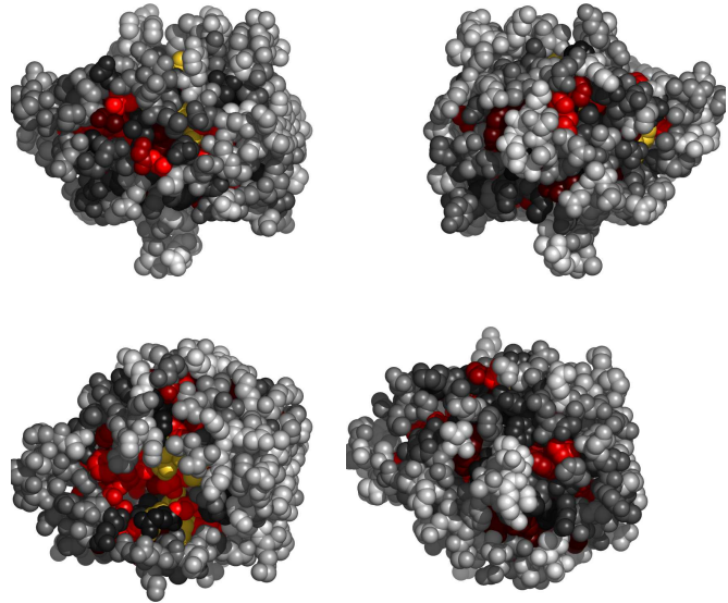
Fig. 1. Residues 16-132 in 2oq5A colored by their relative importance. (See Appendix, Fig.7, for the coloring scheme.) Note that some residues in 2oq5A carry insertion code.
