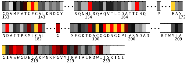
Fig. 2. Residues 133-244 in 2oq5A colored by their relative importance. (See Appendix, Fig.7, for the coloring scheme.) Note that some residues in 2oq5A carry insertion code.
