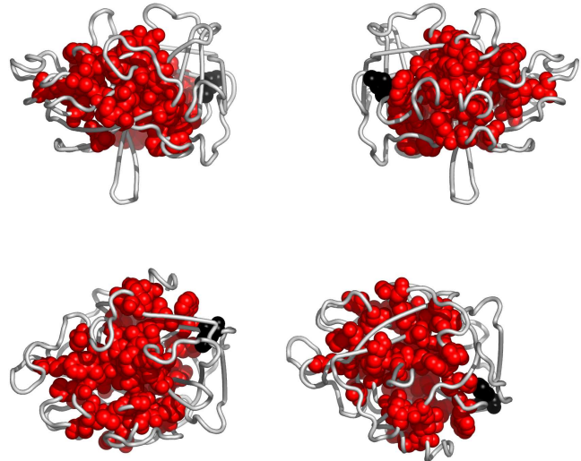
Fig. 4. Residues in 2oq5A, colored according to the cluster they belong to: red, followed by blue and yellow are the largest clusters (see Appendix for the coloring scheme). Clockwise: front, back, top and bottom views. The corresponding Pymol script is attached.
