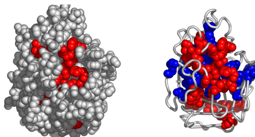
Fig. 5. Residues in 2oq5A, at the interface with benzamidine, colored by their relative importance. The ligand (benzamidine) is colored green. Atoms further than 30 Å away from the geometric center of the ligand, as well as on the line of sight to the ligand were removed. (See Appendix for the coloring scheme for the protein chain 2oq5A.)
