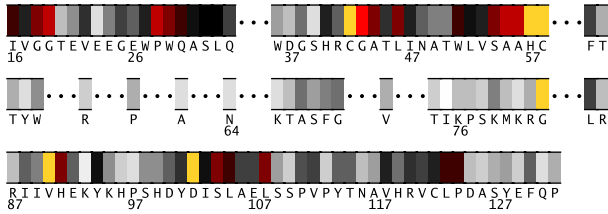
Fig. 1. Residues 16-132 in 2oq5A colored by their relative importance. (See Appendix, Fig.7, for the coloring scheme.) Note that some residues in 2oq5A carry insertion code.
