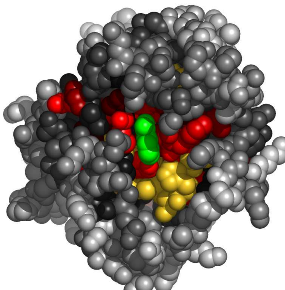
Fig. 5. Residues in 2oq5A, at the interface with benzamidine, colored by their relative importance. The ligand (benzamidine) is colored green. Atoms further than 30 Å away from the geometric center of the ligand, as well as on the line of sight to the ligand were removed. (See Appendix for the coloring scheme for the protein chain 2oq5A.)
