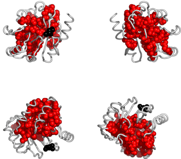
Fig. 3. Residues in 2ox1A, colored according to the cluster they belong to: red, followed by blue and yellow are the largest clusters (see Appendix for the coloring scheme). Clockwise: front, back, top and bottom views. The corresponding Pymol script is attached.
