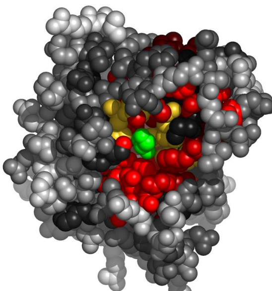
Fig. 4. Residues in 2ox1A, at the interface with glycerol, colored by their relative importance. The ligand (glycerol) is colored green. Atoms further than 30 Å away from the geometric center of the ligand, as well as on the line of sight to the ligand were removed. (See Appendix for the coloring scheme for the protein chain 2ox1A.)
