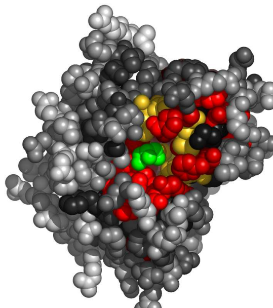
Fig. 5. Residues in 2ox1A, at the interface with glycerol, colored by their relative importance. The ligand (glycerol) is colored green. Atoms further than 30Å away from the geometric center of the ligand, as well as on the line of sight to the ligand were removed. (See Appendix for the coloring scheme for the protein chain 2ox1A.)
