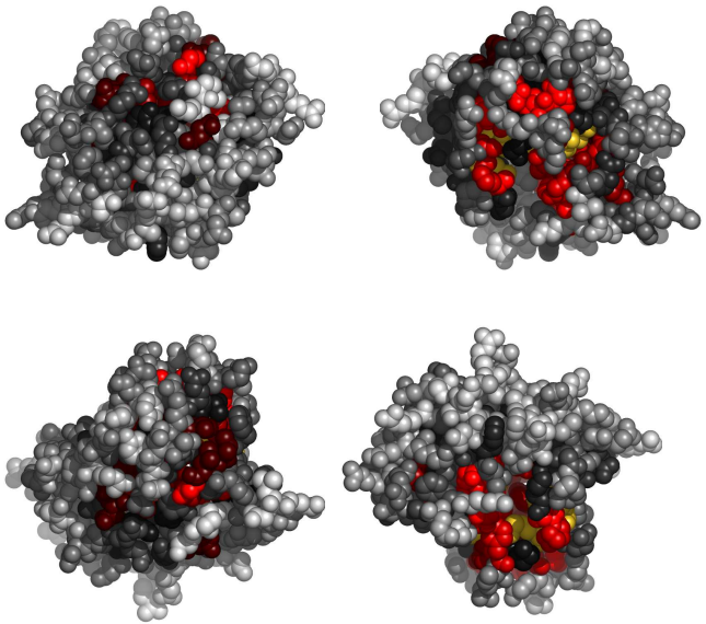
Fig. 2. Residues in 2ox1A, colored by their relative importance. Clockwise: front, back, top and bottom views.
