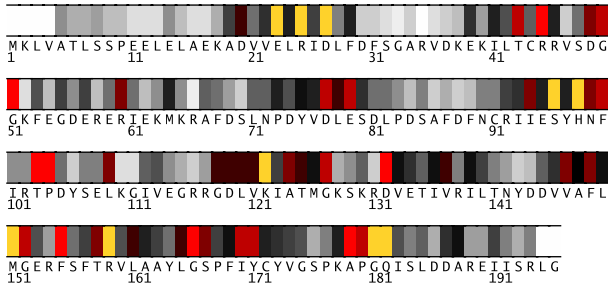
Fig. 1. Residues 1-196 in 2ox1A colored by their relative importance. (See Appendix, Fig.7, for the coloring scheme.)
