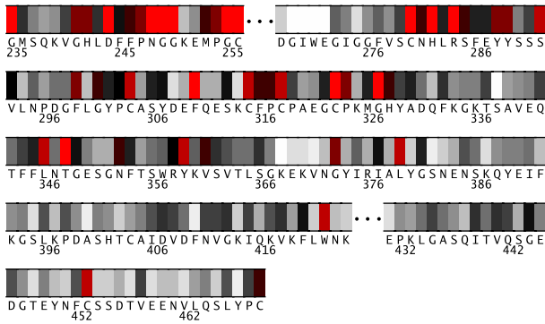
Fig. 2. Residues 235-469 in 20xeA colored by their relative importance. (See Appendix, Fig.9, for the coloring scheme.)
