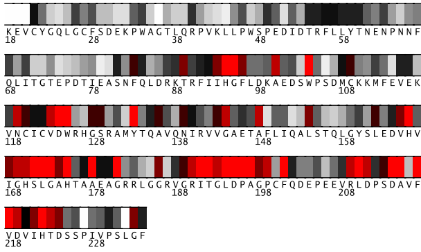
Fig. 1. Residues 18-234 in 20xeA colored by their relative importance. (See Appendix, Fig.9, for the coloring scheme.)
