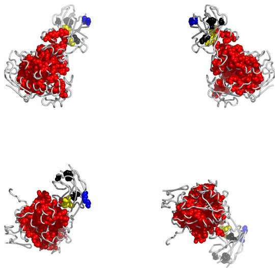
Fig. 4. Residues in 20xA, colored according to the cluster they belong to: red, followed by blue and yellow are the largest clusters (see Appendix for the coloring scheme). Clockwise: front, back, top and bottom views. The corresponding Pymol script is attached.
