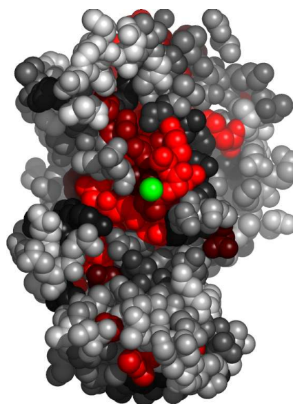
Fig. 5. Residues in 20xA, at the interface with chloride ion, colored by their relative importance. The ligand (chloride ion) is colored green. Atoms further than 30 Å away from the geometric center of the ligand, as well as on the line of sight to the ligand were removed. (See Appendix for the coloring scheme for the protein chain 20xA.)
