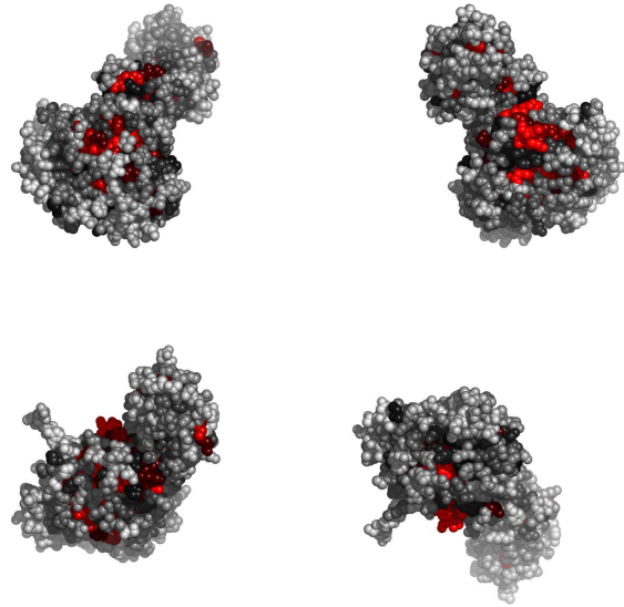
Fig. 3. Residues in 20xeA, colored by their relative importance. Clockwise: front, back, top and bottom views.
