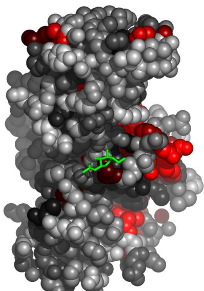
Fig. 6. Residues in 2oxeA, at the interface with NAG, colored by their relative importance. The ligand (NAG) is colored green. Atoms further than 30Å away from the geometric center of the ligand, as well as on the line of sight to the ligand were removed. (See Appendix for the coloring scheme for the protein chain 2oxeA.)
