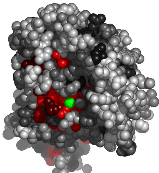
Fig. 7. Residues in 20xeA, at the interface with calcium ion, colored by their relative importance. The ligand (calcium ion) is colored green. Atoms further than 30Å away from the geometric center of the ligand, as well as on the line of sight to the ligand were removed. (See Appendix for the coloring scheme for the protein chain 20xeA.)
