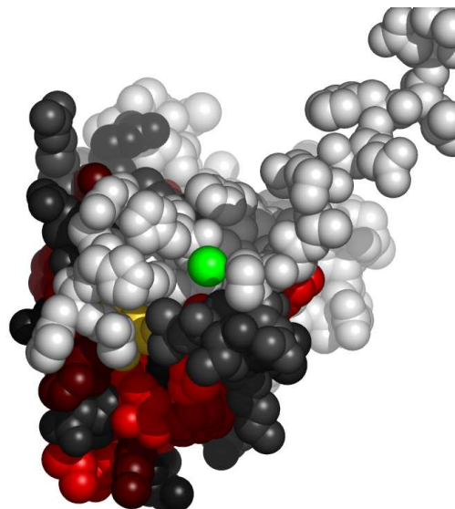
Fig. 5. Residues in 2pf1B, at the interface with chloride ion, colored by their relative importance. The ligand (chloride ion) is colored green. Atoms further than 30Å away from the geometric center of the ligand, as well as on the line of sight to the ligand were removed. (See Appendix for the coloring scheme for the protein chain 2pf1B.)
