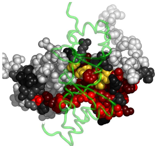
Fig. 4. Residues in 2pf1B, at the interface with 2pf1A, colored by their relative importance. 2pf1A is shown in backbone representation (See Appendix for the coloring scheme for the protein chain 2pf1B.)
