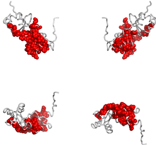
Fig. 2. Residues in 2pfiB, colored by their relative importance. Clockwise: front, back, top and bottom views.
