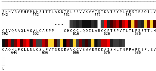
Fig. 1. Residues 542-693 in 2pfiB colored by their relative importance. (See Appendix, Fig.8, for the coloring scheme.)
