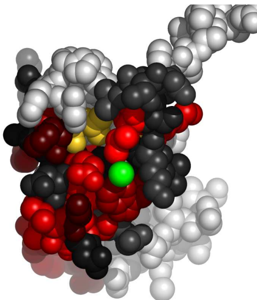
Fig. 6. Residues in 2pfiB, at the interface with chloride ion, colored by their relative importance. The ligand (chloride ion) is colored green. Atoms further than 30Å away from the geometric center of the ligand, as well as on the line of sight to the ligand were removed. (See Appendix for the coloring scheme for the protein chain 2pfiB.)
