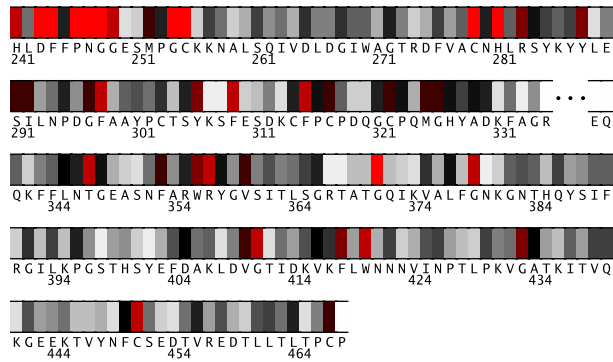
Fig. 2. Residues 241-468 in 2pplA colored by their relative importance. (See Appendix, Fig.12, for the coloring scheme.)
