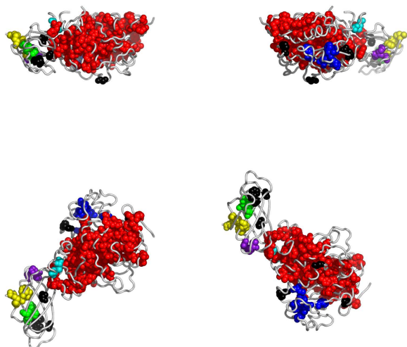
Fig. 4. Residues in 2pplA, colored according to the cluster they belong to: red, followed by blue and yellow are the largest clusters (see Appendix for the coloring scheme). Clockwise: front, back, top and bottom views. The corresponding Pymol script is attached.
