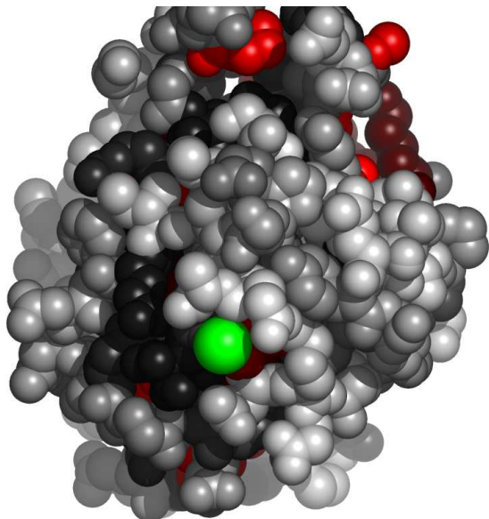
Fig. 6. Residues in 2pplA, at the interface with sodium ion, colored by their relative importance. The ligand (sodium ion) is colored green. Atoms further than 30Å away from the geometric center of the ligand, as well as on the line of sight to the ligand were removed. (See Appendix for the coloring scheme for the protein chain 2pplA.)
