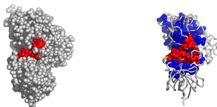
Fig. 10. Another possible active surface on the chain 2pplA. The larger cluster it belongs to is shown in blue.
