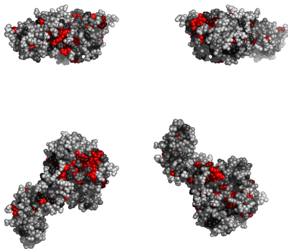
Fig. 3. Residues in 2pplA, colored by their relative importance. Clockwise: front, back, top and bottom views.
