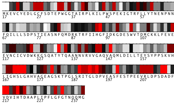
Fig. 1. Residues 17-240 in 2pplA colored by their relative importance. (See Appendix, Fig.12, for the coloring scheme.)
