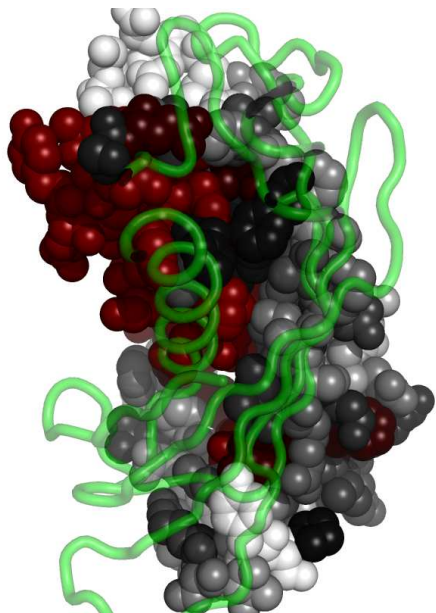
Fig. 5. Residues in 2pzhA, at the interface with 2pzhB, colored by their relative importance. 2pzhB is shown in backbone representation (See Appendix for the coloring scheme for the protein chain 2pzhA.)
