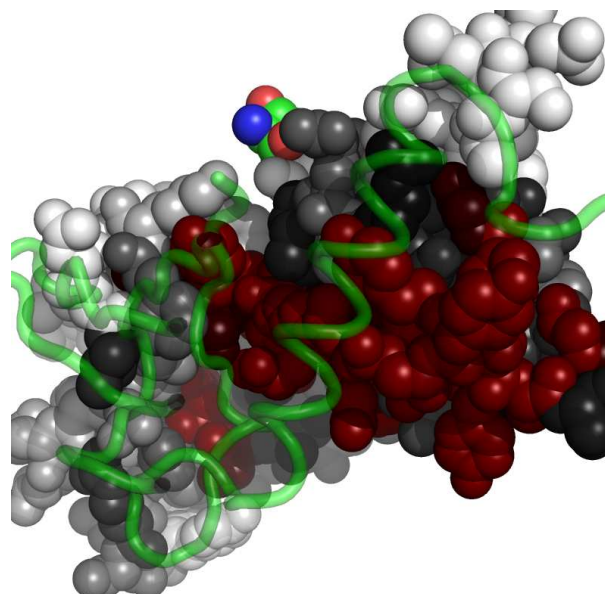
Fig. 4. Residues in 2pzhA, at the interface with 2pzhD, colored by their relative importance. 2pzhD is shown in backbone representation (See Appendix for the coloring scheme for the protein chain 2pzhA.)
