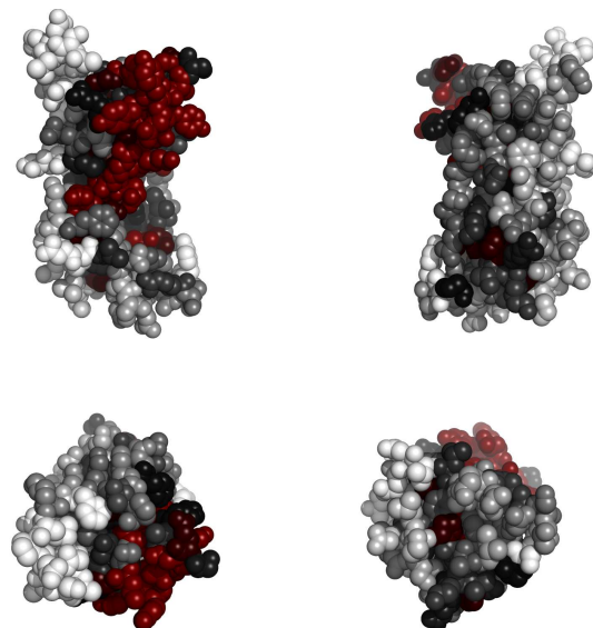
Fig. 2. Residues in 2pzhA, colored by their relative importance. Clockwise: front, back, top and bottom views.
