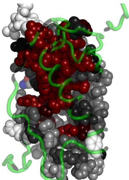
Fig. 6. Residues in 2pzhA, at the interface with 2pzhC, colored by their relative importance. 2pzhC is shown in backbone representation (See Appendix for the coloring scheme for the protein chain 2pzhA.)
