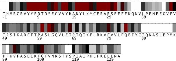
Fig. 1. Residues -1-132 in 2pzhA colored by their relative importance. (See Appendix, Fig.7, for the coloring scheme.)
