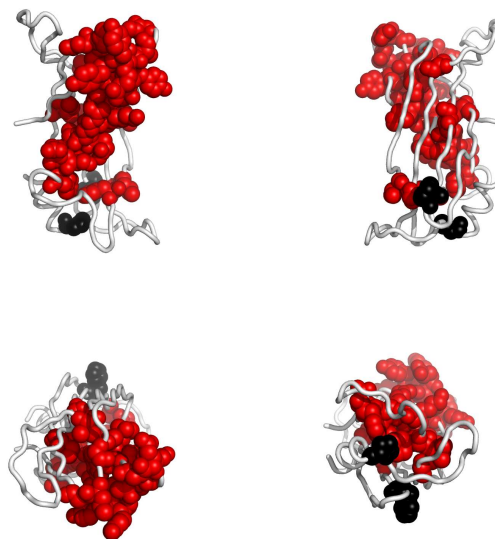
Fig. 3. Residues in 2pzhA, colored according to the cluster they belong to: red, followed by blue and yellow are the largest clusters (see Appendix for the coloring scheme). Clockwise: front, back, top and bottom views. The corresponding Pymol script is attached.
