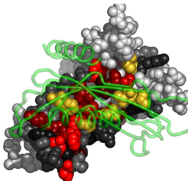
Fig. 6. Residues in 2qq2C, at the interface with 2qq2K, colored by their relative importance. 2qq2K is shown in backbone representation (See Appendix for the coloring scheme for the protein chain 2qq2C.)
