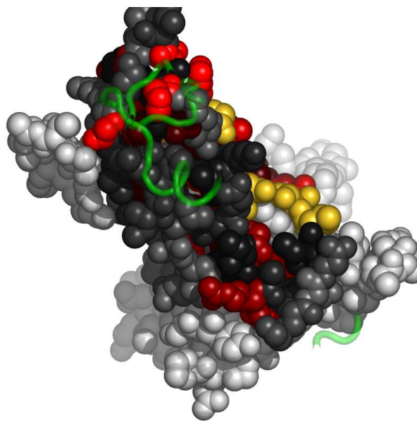
Fig. 5. Residues in 2qq2C, at the interface with 2qq2E, colored by their relative importance. 2qq2E is shown in backbone representation (See Appendix for the coloring scheme for the protein chain 2qq2C.)
