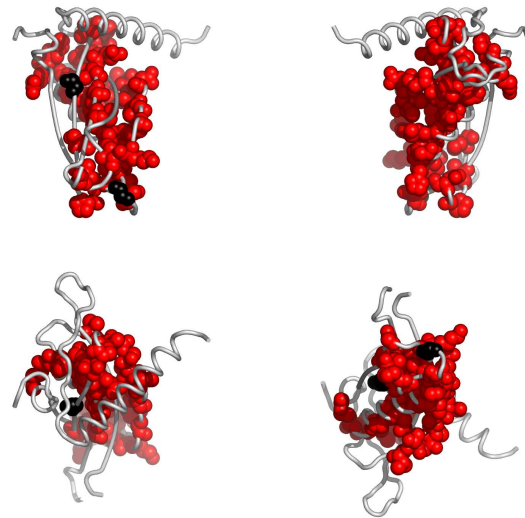
Fig. 3. Residues in 2qq2C, colored according to the cluster they belong to: red, followed by blue and yellow are the largest clusters (see Appendix for the coloring scheme). Clockwise: front, back, top and bottom views. The corresponding Pymol script is attached.
