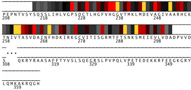
Fig. 1. Residues 208-365 in 2qq2C colored by their relative importance. (See Appendix, Fig.9, for the coloring scheme.)
