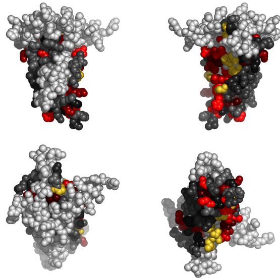
Fig. 2. Residues in 2qq2C, colored by their relative importance. Clockwise: front, back, top and bottom views.
