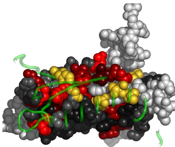
Fig. 6. Residues in 2qq2C, at the interface with 2qq2K, colored by their relative importance. 2qq2K is shown in backbone representation (See Appendix for the coloring scheme for the protein chain 2qq2C.)
