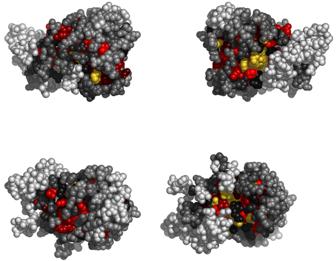
Fig. 1. Residues 675-817 in 2rf9A colored by their relative importance. (See Appendix, Fig.7, for the coloring scheme.)
