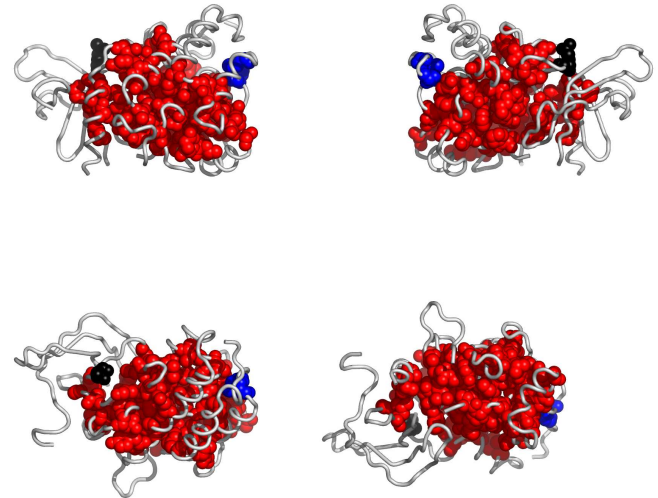
Fig. 4. Residues in 2rf9A, colored according to the cluster they belong to: red, followed by blue and yellow are the largest clusters (see Appendix for the coloring scheme). Clockwise: front, back, top and bottom views. The corresponding Pymol script is attached.
