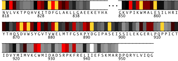
Fig. 2. Residues 818-959 in 2rf9A colored by their relative importance. (See Appendix, Fig.7, for the coloring scheme.)
