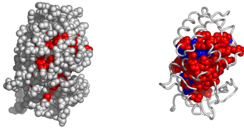
Fig. 6. A possible active surface on the chain 2rf9A. The larger cluster it belongs to is shown in blue.
