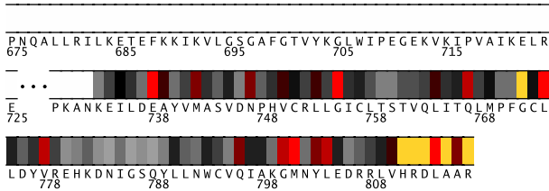
Fig. 1. Residues 675-817 in 2rf9A colored by their relative importance. (See Appendix, Fig.7, for the coloring scheme.)
