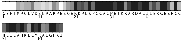
Fig. 1. Residues 1-67 in 2rn9A colored by their relative importance. (See Appendix, Fig.4, for the coloring scheme.)
