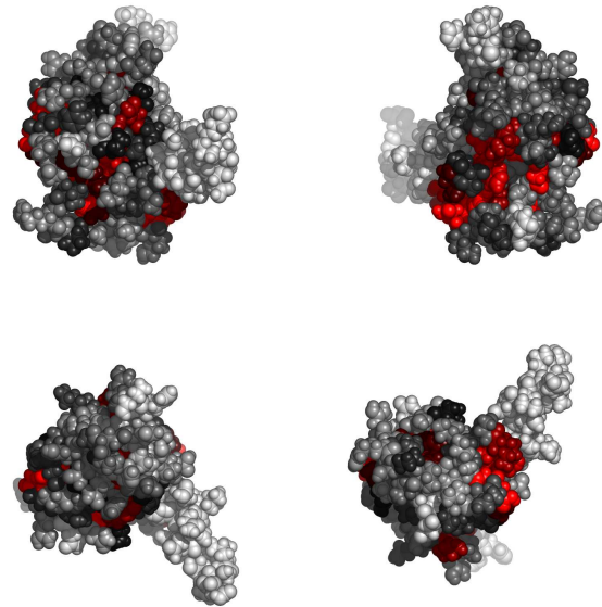
Fig. 2. Residues in 2rqaA, colored by their relative importance. Clockwise: front, back, top and bottom views.
