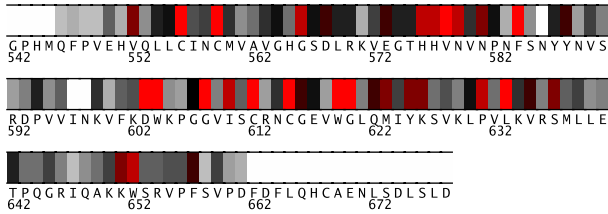
Fig. 1. Residues 542-678 in 2rqaA colored by their relative importance. (See Appendix, Fig.6, for the coloring scheme.)
