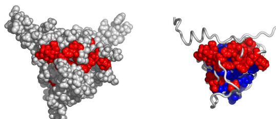
Fig. 5. A possible active surface on the chain 2rqaA. The larger cluster it belongs to is shown in blue.
