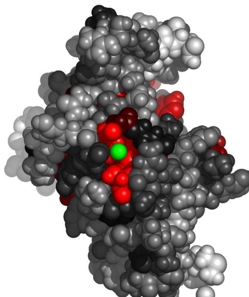
Fig. 4. Residues in 2rqaA, at the interface with zinc ion, colored by their relative importance. The ligand (zinc ion) is colored green. Atoms further than 30 Å away from the geometric center of the ligand, as well as on the line of sight to the ligand were removed. (See Appendix for the coloring scheme for the protein chain 2rqaA.)
