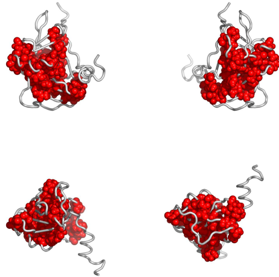
Fig. 3. Residues in 2rqaA, colored according to the cluster they belong to: red, followed by blue and yellow are the largest clusters (see Appendix for the coloring scheme). Clockwise: front, back, top and bottom views. The corresponding Pymol script is attached.
