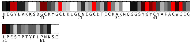
Fig. 1. Residues 1-65 in 2sn3A colored by their relative importance. (See Appendix, Fig.5, for the coloring scheme.)
