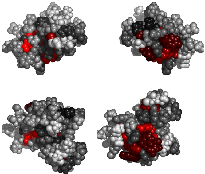
Fig. 2. Residues in 2sn3A, colored by their relative importance. Clockwise: front, back, top and bottom views.
