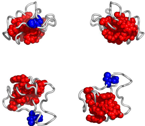
Fig. 3. Residues in 2sn3A, colored according to the cluster they belong to: red, followed by blue and yellow are the largest clusters (see Appendix for the coloring scheme). Clockwise: front, back, top and bottom views. The corresponding Pymol script is attached.
