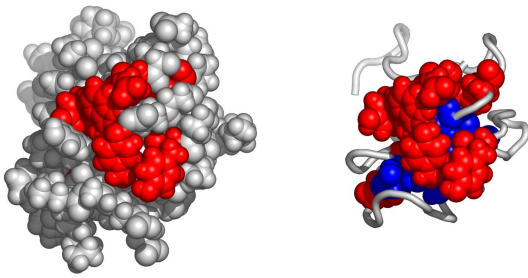
Fig. 4. A possible active surface on the chain 2sn3A. The larger cluster it belongs to is shown in blue.
