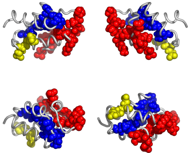
Fig. 3. Residues in 2v6zM, colored according to the cluster they belong to: red, followed by blue and yellow are the largest clusters (see Appendix for the coloring scheme). Clockwise: front, back, top and bottom views. The corresponding Pymol script is attached.
