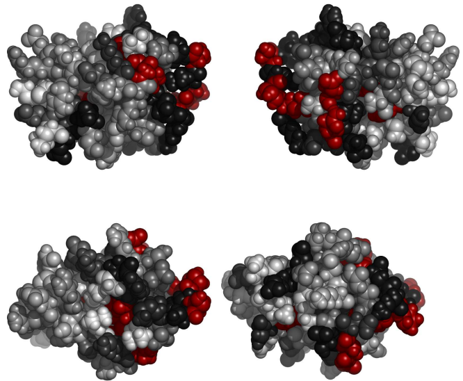
Fig. 1. Residues 25-99 in 2v6zM colored by their relative importance. (See Appendix, Fig.5, for the coloring scheme.)
