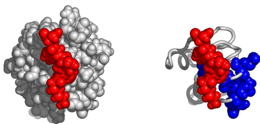
Fig. 4. A possible active surface on the chain 2v6zM. The larger cluster it belongs to is shown in blue.
