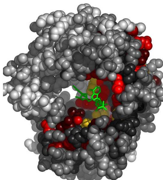
Fig. 5. Residues in 2vn8A, at the interface with NDP, colored by their relative importance. The ligand (NDP) is colored green. Atoms further than 30Å away from the geometric center of the ligand, as well as on the line of sight to the ligand were removed. (See Appendix for the coloring scheme for the protein chain 2vn8A.)
