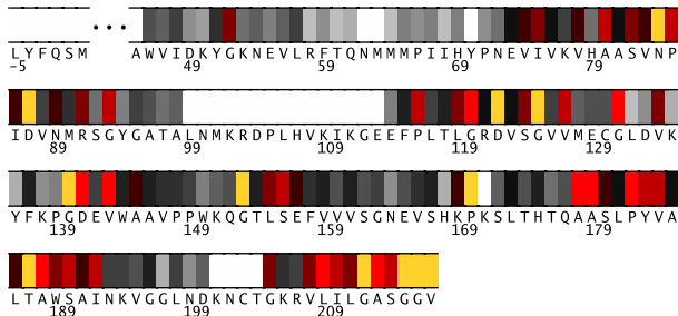
Fig. 1. Residues -5-217 in 2vn8A colored by their relative importance. (See Appendix, Fig.8, for the coloring scheme.)
