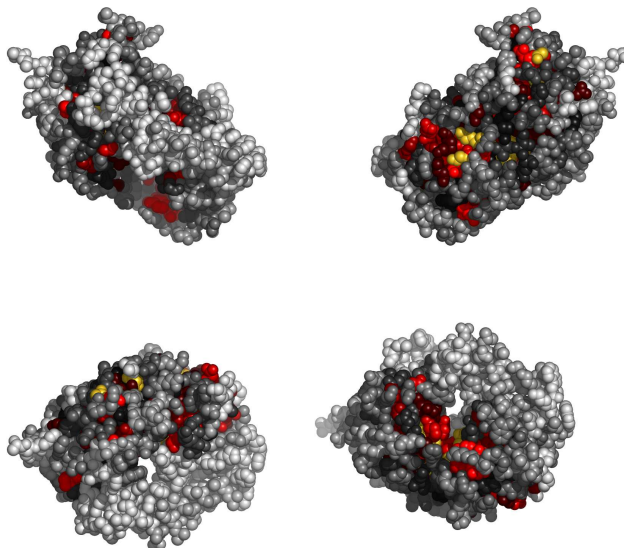
Fig. 3. Residues in 2vn8A, colored by their relative importance. Clockwise: front, back, top and bottom views.
