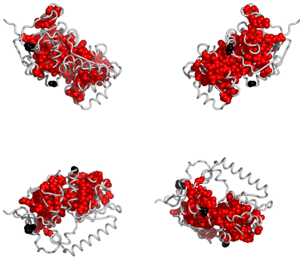
Fig. 4. Residues in 2vn8A, colored according to the cluster they belong to: red, followed by blue and yellow are the largest clusters (see Appendix for the coloring scheme). Clockwise: front, back, top and bottom views. The corresponding Pymol script is attached.
