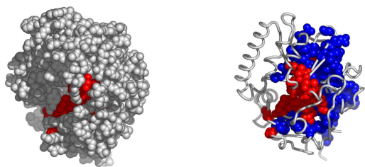
Fig. 6. A possible active surface on the chain 2vn8A. The larger cluster it belongs to is shown in blue.
