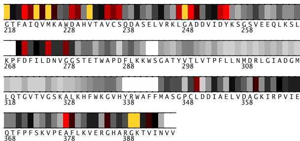
Fig. 2. Residues 218-396 in 2vn8A colored by their relative importance. (See Appendix, Fig.8, for the coloring scheme.)
