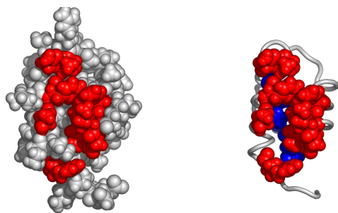
Fig. 5. A possible active surface on the chain 2w84A. The larger cluster it belongs to is shown in blue.
