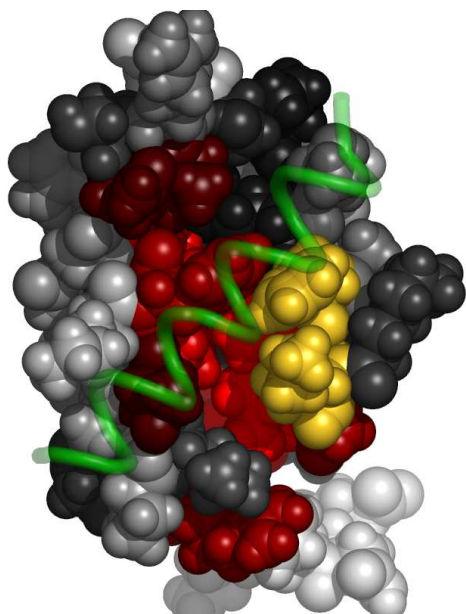
Fig. 4. Residues in 2w84A, at the interface with 2w84B, colored by their relative importance. 2w84B is shown in backbone representation (See Appendix for the coloring scheme for the protein chain 2w84A.)
