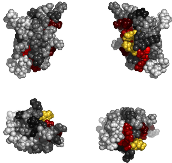
Fig. 2. Residues in 2w84A, colored by their relative importance. Clockwise: front, back, top and bottom views.
