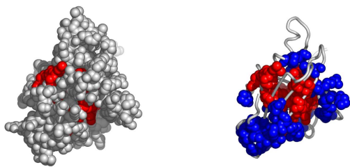
Fig. 5. A possible active surface on the chain 2wewA. The larger cluster it belongs to is shown in blue.
