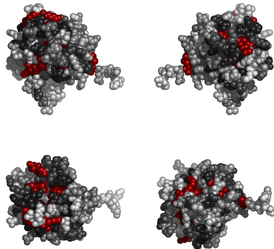
Fig. 1. Residues 18-187 in 2wewA colored by their relative importance. (See Appendix, Fig.6, for the coloring scheme.)
