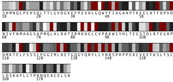
Fig. 1. Residues 18-187 in 2wewA colored by their relative importance. (See Appendix, Fig.6, for the coloring scheme.)
