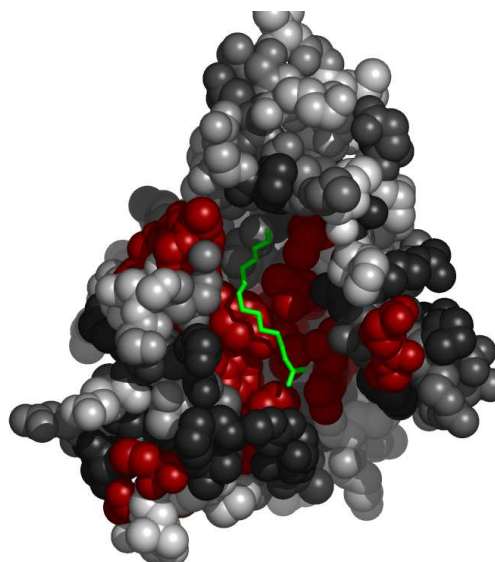
Fig. 4. Residues in 2wewA, at the interface with myristic acid, colored by their relative importance. The ligand (myristic acid) is colored green. Atoms further than 30 Å away from the geometric center of the ligand, as well as on the line of sight to the ligand were removed. (See Appendix for the coloring scheme for the protein chain 2wewA.)
