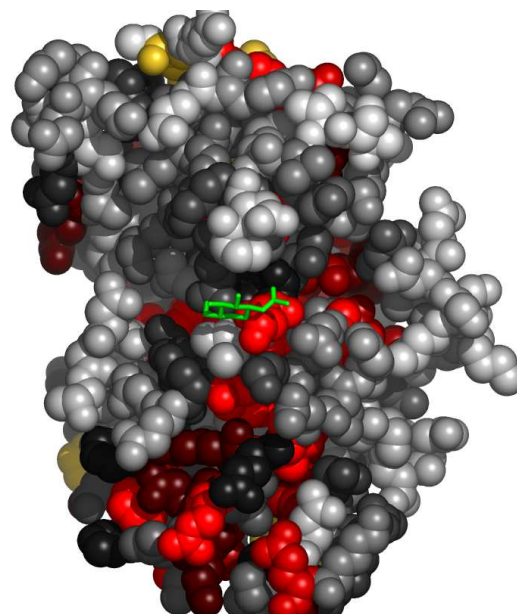
Fig. 5. Residues in 2wjwA, at the interface with NAG, colored by their relative importance. The ligand (NAG) is colored green. Atoms further than 30 Å away from the geometric center of the ligand, as well as on the line of sight to the ligand were removed. (See Appendix for the coloring scheme for the protein chain 2wjwA.)
