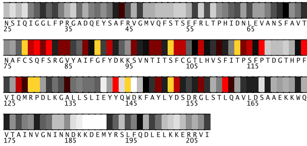
Fig. 1. Residues 25-208 in 2wjwA colored by their relative importance. (See Appendix, Fig.11, for the coloring scheme.)
