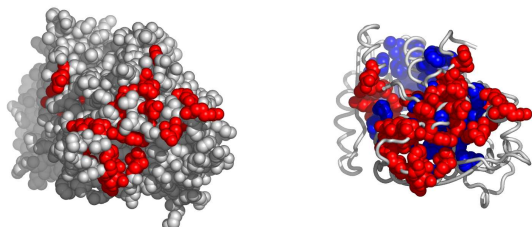
Fig. 10. Another possible active surface on the chain 2wjwA. The larger cluster it belongs to is shown in blue.
