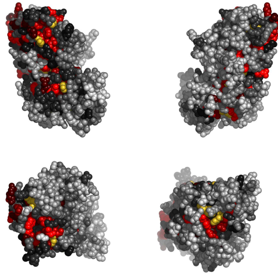
Fig. 3. Residues in 2wjwA, colored by their relative importance. Clockwise: front, back, top and bottom views.
