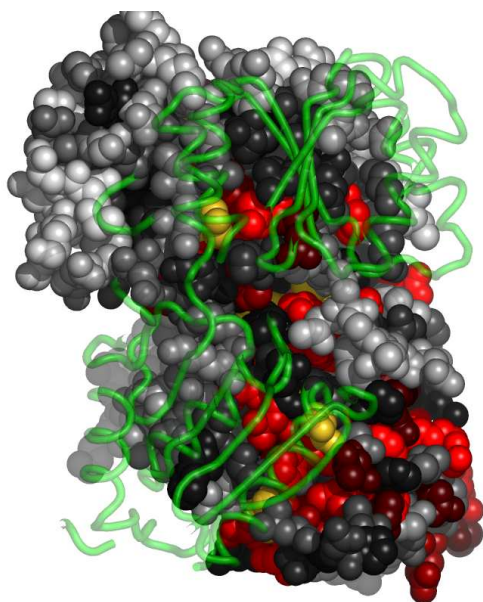
Fig. 8. Residues in 2wjwA, at the interface with 2wjwA1, colored by their relative importance. 2wjwA1 is shown in backbone representation (See Appendix for the coloring scheme for the protein chain 2wjwA.)
