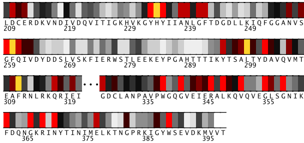
Fig. 2. Residues 209-398 in 2wjwA colored by their relative importance. (See Appendix, Fig.11, for the coloring scheme.)
