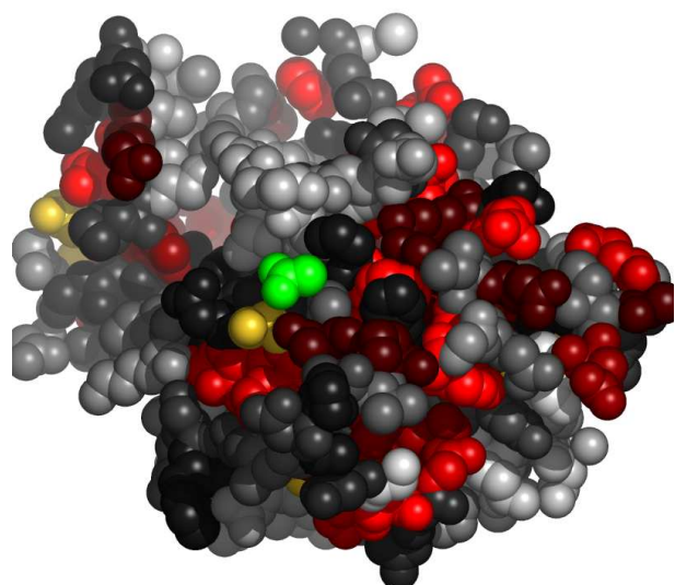
Fig. 6. Residues in 2wjwA, at the interface with acetate ion, colored by their relative importance. The ligand (acetate ion) is colored green. Atoms further than 30Å away from the geometric center of the ligand, as well as on the line of sight to the ligand were removed. (See Appendix for the coloring scheme for the protein chain 2wjwA.)
