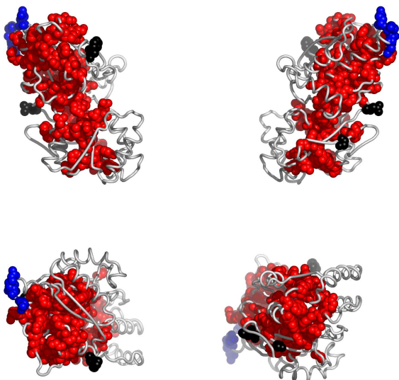
Fig. 4. Residues in 2wjwA, colored according to the cluster they belong to: red, followed by blue and yellow are the largest clusters (see Appendix for the coloring scheme). Clockwise: front, back, top and bottom views. The corresponding Pymol script is attached.
