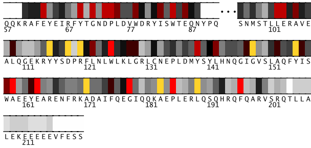
Fig. 1. Residues 57-220 in 2wviA colored by their relative importance. (See Appendix, Fig.6, for the coloring scheme.)
