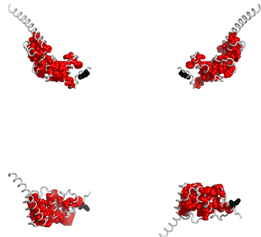
Fig. 2. Residues in 2wviA, colored by their relative importance. Clockwise: front, back, top and bottom views.
