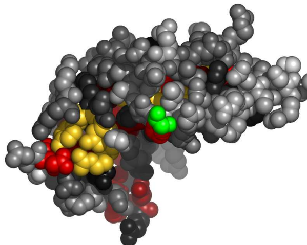
Fig. 4. Residues in 2wviA, at the interface with 1,2-ethanediol, colored by their relative importance. The ligand (1,2-ethanediol) is colored green. Atoms further than 30Å away from the geometric center of the ligand, as well as on the line of sight to the ligand were removed. (See Appendix for the coloring scheme for the protein chain 2wviA.)
