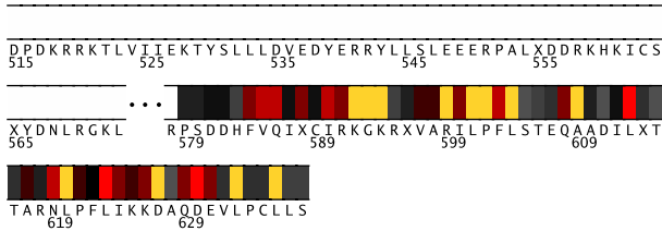
Fig. 1. Residues 515-638 in 2xeqC colored by their relative importance. (See Appendix, Fig.9, for the coloring scheme.)
