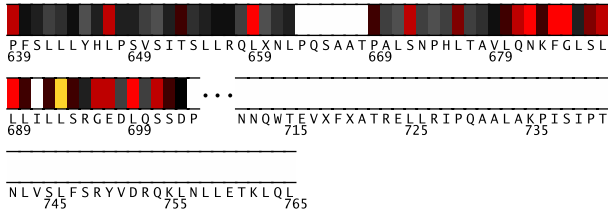
Fig. 2. Residues 639-765 in 2xeqC colored by their relative importance. (See Appendix, Fig.9, for the coloring scheme.)
