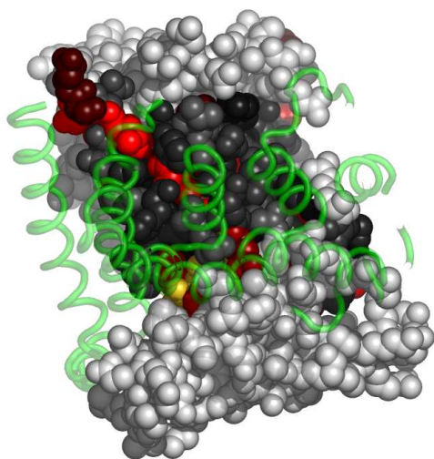
Fig. 6. Residues in 2xeqC, at the interface with 2xeqB, colored by their relative importance. 2xeqB is shown in backbone representation (See Appendix for the coloring scheme for the protein chain 2xeqC.)
