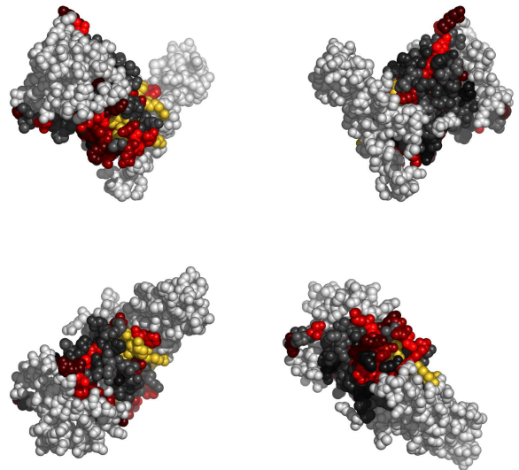
Fig. 3. Residues in 2xeqC, colored by their relative importance. Clockwise: front, back, top and bottom views.
