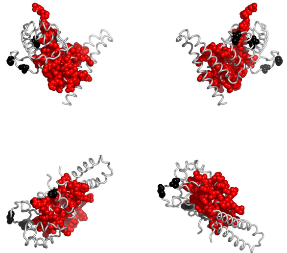
Fig. 4. Residues in 2xeqC, colored according to the cluster they belong to: red, followed by blue and yellow are the largest clusters (see Appendix for the coloring scheme). Clockwise: front, back, top and bottom views. The corresponding Pymol script is attached.
