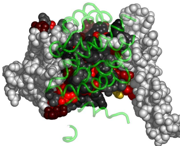
Fig. 7. Residues in 2xeqC, at the interface with 2xeqA, colored by their relative importance. 2xeqA is shown in backbone representation (See Appendix for the coloring scheme for the protein chain 2xeqC.)
