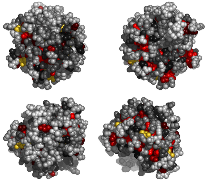
Fig. 3. Residues in 2xn4A, colored by their relative importance. Clockwise: front, back, top and bottom views.
