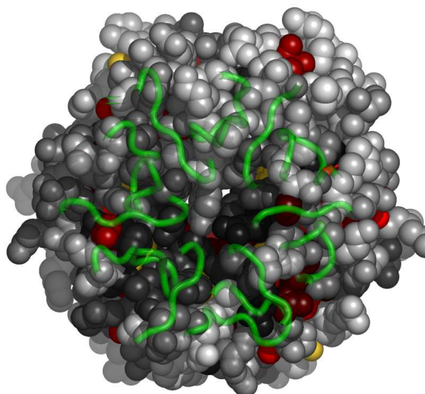
Fig. 7. Residues in 2xn4A, at the interface with 2xn4B, colored by their relative importance. 2xn4B is shown in backbone representation (See Appendix for the coloring scheme for the protein chain 2xn4A.)
