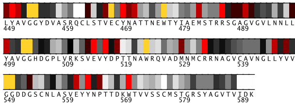
Fig. 2. Residues 449-591 in 2xn4A colored by their relative importance. (See Appendix, Fig.9, for the coloring scheme.)
