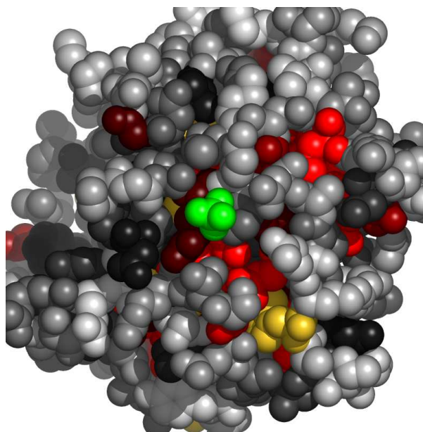
Fig. 6. Residues in 2xn4A, at the interface with sulfate ion, colored by their relative importance. The ligand (sulfate ion) is colored green. Atoms further than 30Å away from the geometric center of the ligand, as well as on the line of sight to the ligand were removed. (See Appendix for the coloring scheme for the protein chain 2xn4A.)
