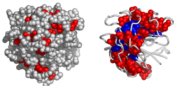
Fig. 8. A possible active surface on the chain 2xn4A. The larger cluster it belongs to is shown in blue.
