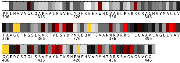
Fig. 1. Residues 306-448 in 2xn4A colored by their relative importance. (See Appendix, Fig.9, for the coloring scheme.)
