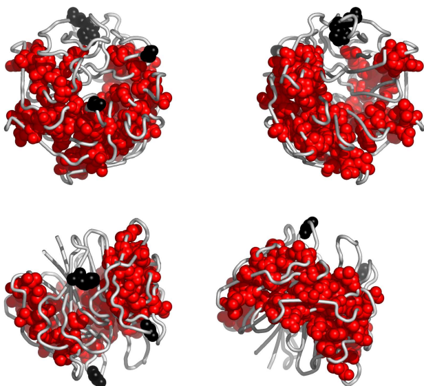
Fig. 4. Residues in 2xn4A, colored according to the cluster they belong to: red, followed by blue and yellow are the largest clusters (see Appendix for the coloring scheme). Clockwise: front, back, top and bottom views. The corresponding Pymol script is attached.
