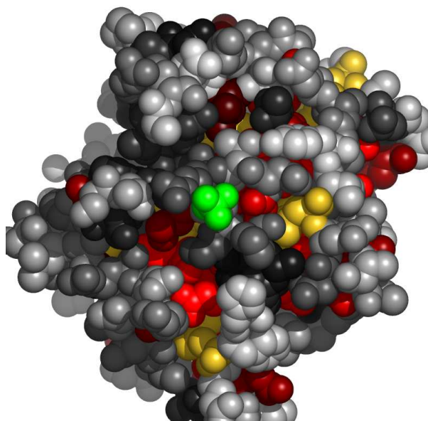
Fig. 5. Residues in 2xn4A, at the interface with sulfate ion, colored by their relative importance. The ligand (sulfate ion) is colored green. Atoms further than 30 Å away from the geometric center of the ligand, as well as on the line of sight to the ligand were removed. (See Appendix for the coloring scheme for the protein chain 2xn4A.)
