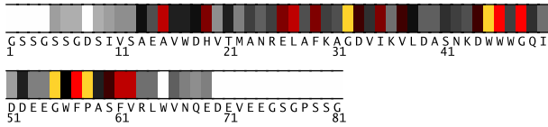
Fig. 1. Residues 1-81 in 2ysqA colored by their relative importance. (See Appendix, Fig.5, for the coloring scheme.)
