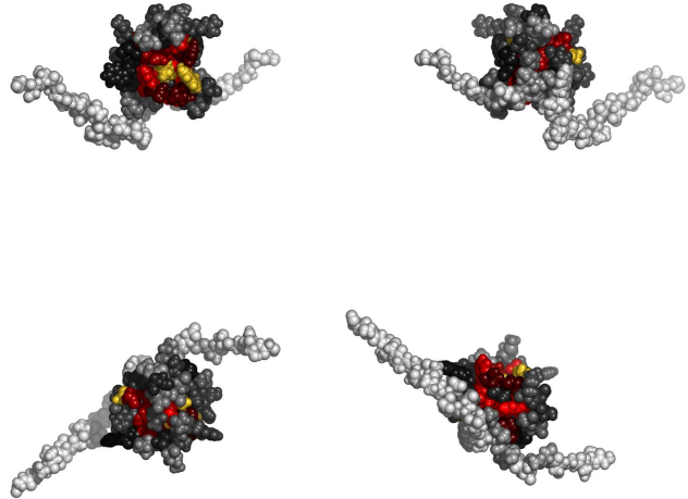
Fig. 1. Residues 1-81 in 2ysqA colored by their relative importance. (See Appendix, Fig.5, for the coloring scheme.)
