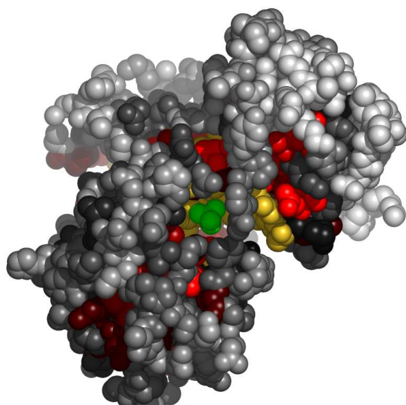
Fig. 5. Residues in 2zpaB, at the interface with sulfate ion, colored by their relative importance. The ligand (sulfate ion) is colored green. Atoms further than 30 Å away from the geometric center of the ligand, as well as on the line of sight to the ligand were removed. (See Appendix for the coloring scheme for the protein chain 2zpaB.)
