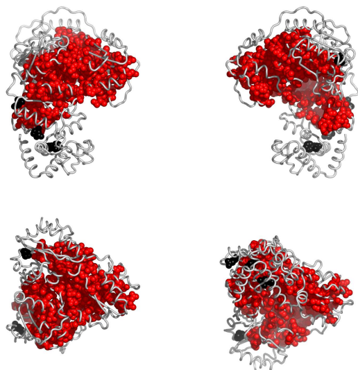
Fig. 4. Residues in 2zpaB, colored according to the cluster they belong to: red, followed by blue and yellow are the largest clusters (see Appendix for the coloring scheme). Clockwise: front, back, top and bottom views. The corresponding Pymol script is attached.
