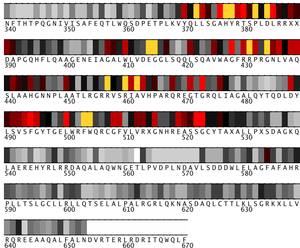
Fig. 2. Residues 340-670 in 2zpaB colored by their relative importance. (See Appendix, Fig.7, for the coloring scheme.)
