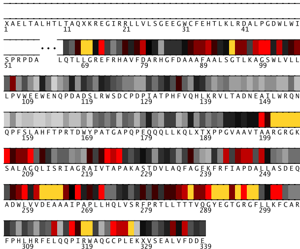
Fig. 1. Residues 1-339 in 2zpaB colored by their relative importance. (See Appendix, Fig.7, for the coloring scheme.)
