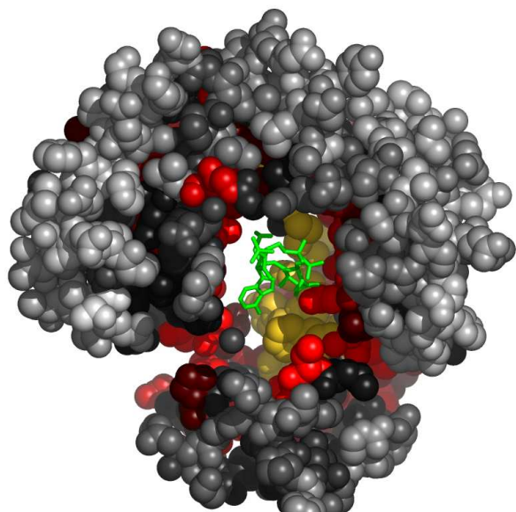
Fig. 6. Residues in 2zpaB, at the interface with acetyl coenzyme *a, colored by their relative importance. The ligand (acetyl coenzyme *a) is colored green. Atoms further than 30 Å away from the geometric center of the ligand, as well as on the line of sight to the ligand were removed. (See Appendix for the coloring scheme for the protein chain 2zpaB.)
