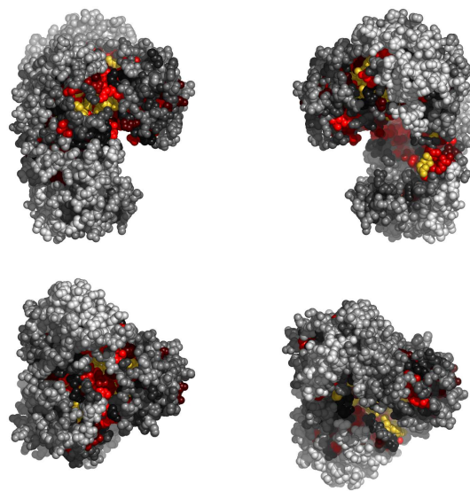
Fig. 3. Residues in 2zpaB, colored by their relative importance. Clockwise: front, back, top and bottom views.
