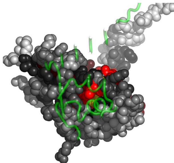
Fig. 4. Residues in 3bimE, at the interface with 3bimF, colored by their relative importance. 3bimF is shown in backbone representation (See Appendix for the coloring scheme for the protein chain 3bimE.)
