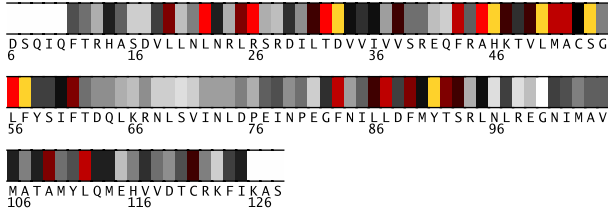
Fig. 1. Residues 6-128 in 3bimE colored by their relative importance. (See Appendix, Fig.9, for the coloring scheme.)
