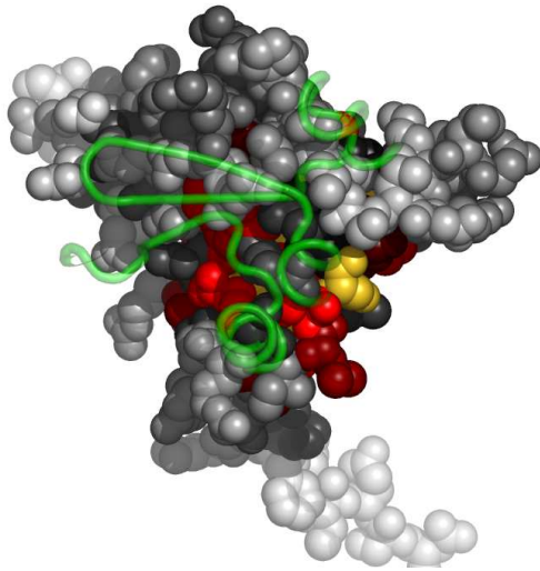
Fig. 7. Residues in 3bimE, at the interface with 3bimC, colored by their relative importance. 3bimC is shown in backbone representation (See Appendix for the coloring scheme for the protein chain 3bimE.)
