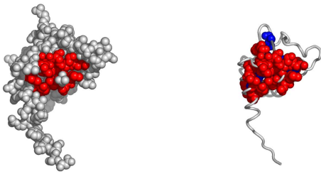
Fig. 8. A possible active surface on the chain 3bimE. The larger cluster it belongs to is shown in blue.
